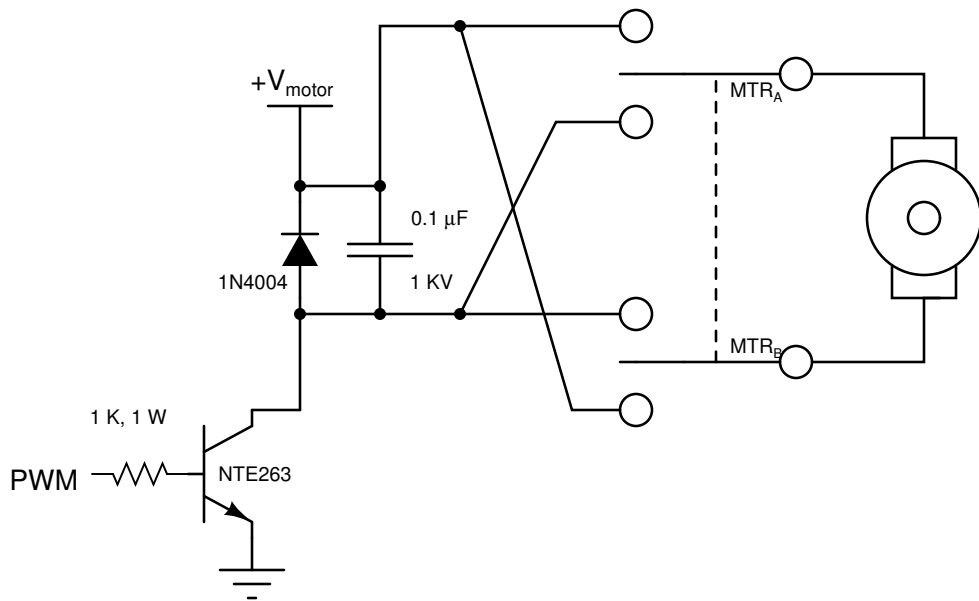
DPDT SWITCH DC MOTOR FWD/REV CIRCUIT
