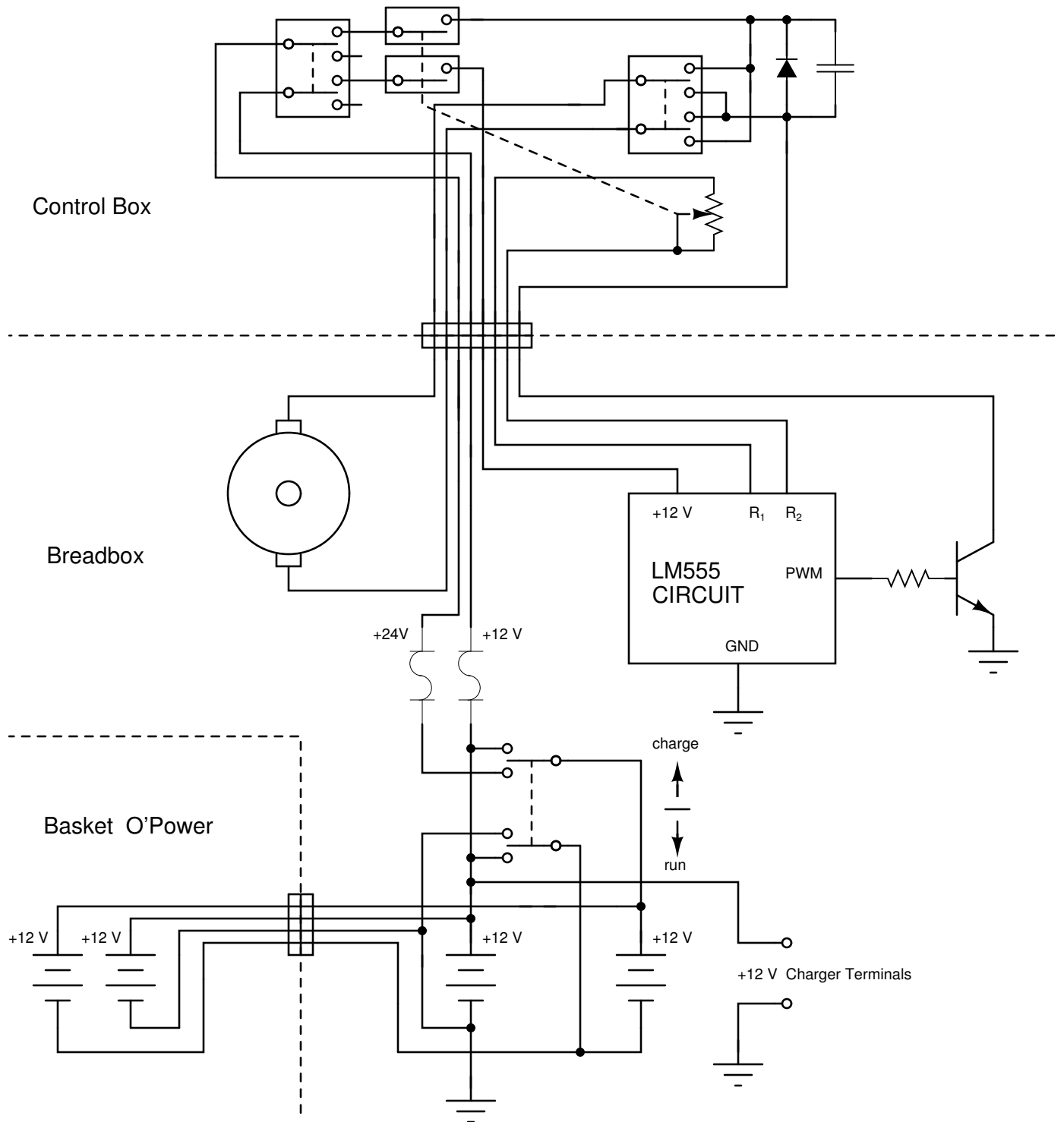
ATAWLC COMPLETE DRIVE AND CONTROL CIRCUIT
