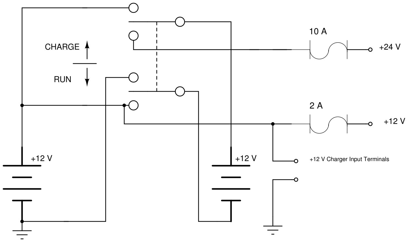
+24V,+12V/+12V RUN/CHARGE DPDT SWITCH CIRCUIT
