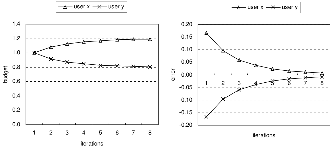
Figure 2: Convergence of iterative algorithm for satisfying power demands.
