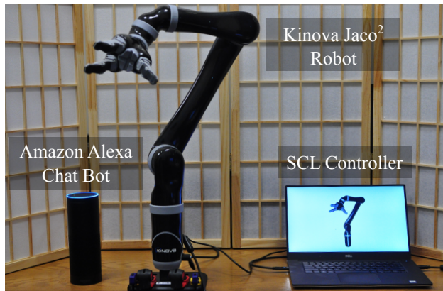
Figure 1: Voice-Activated Robot Motion Synthesis: An Amazon Alexa device translates vocal natural language commands to a structured text representation, which is transmitted over the internet to a Redis database. A Standard Control Library (SCL) controller maps text into analog trajectories in task space, and then computes appropriate control torques to actuate a Kinova Jaco 2 robot.
