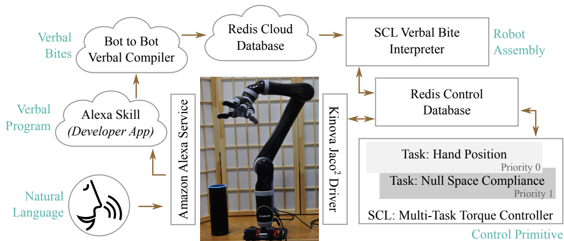
Figure 2: Compiling Natural Language to Robot Motion: Information flow in the Bot to Bot system starts with human natural language (bottom left), which is parsed by Amazon’s Alexa Service and an Alexa Skill application into a verbal program . A Bot to Bot verbal compiler transforms the program to lower level verbal bites , which are further transformed to yet lower level robot assembly commands by the SCL verbal bite interpreter. Finally, a closed-loop multi-task controller runs a control primitive —a set of prioritized tasks with specific goal conditions—that executes the robot assembly code.
