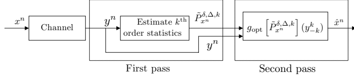
Continuous Context-free(Symbol-by-Symbol) Denoiser [1]
