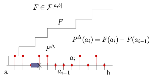
Fig. 1. Quantization of the support of a distribution function, F \in \mathcal{F}^{[a,b]} , \mathcal{A}^\Delta = \{a_i = a + i\Delta, i = 0, \dots, N(\Delta) - 1\} , N(\Delta) is the number of points in the interval [a, b] corresponding to a quantization step-size of \Delta
