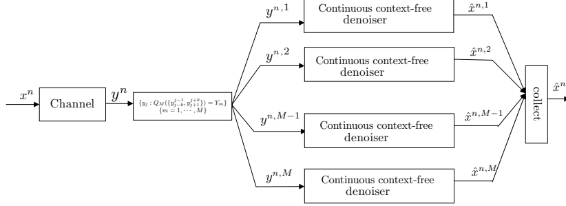
Modified Denoiser
