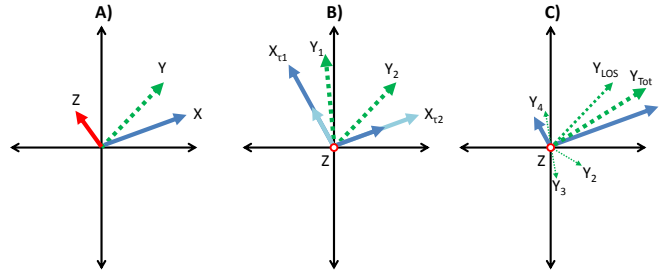
Figure 7: Reference Signal shown in blue (X), interference signal shown in green (Y), residual signal shown in red (Z). A) Effect of delay mismatch on signal cancellation: Delay offsets result in imperfect cancellation. B) 2 fixed delay paths with tunable attenuators: Different attenuator values compensate for different delay values. C) Helps mitigate effects of multipath due to reflections: Picasso is tuned to cancel the aggregate response ( Y_{Tot} ), not just the LOS component.
