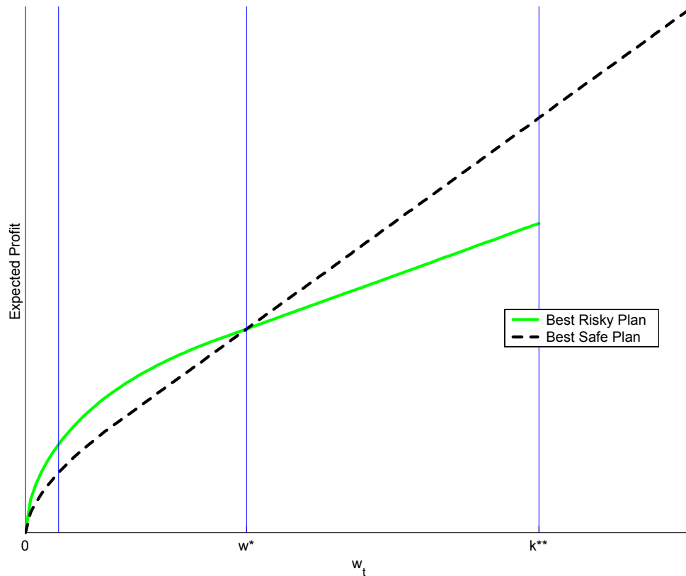
Figure 3.2: Expected profit as a function of internal funds, under the best risky and safe plan.
