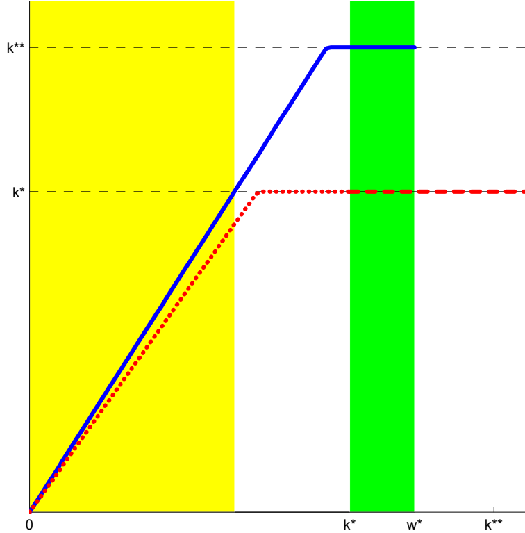
Figure 3.1: Investment and equilibrium regions.
