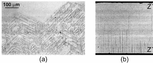
FIGURE 5. (a) Z^- view, (b) Y view of CDW in CLN. ITO electrodes. Optical visualization of etched surface. 0.2-mm-thick sample.
