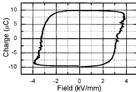
FIGURE 4. Hysteresis loop in MgO:SLN. Liquid electrodes.
