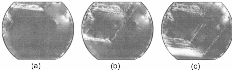
FIGURE 6. CDW in SLN. Time interval from field switch-on: (a) 2.4 s, (b) 2.6 s, (c) 2.8 s. ITO electrodes. E = 4.8 kV/mm. 1-mm-diameter area.
