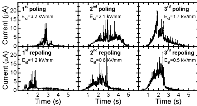
FIGURE 3. Evolution of switching current during cyclic switching in MgO:SLN. Liquid electrodes. E_{\max} = 4 kV/mm.
