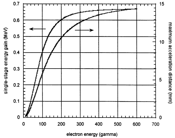
Fig. 2. The dependence of the single-stage energy gain and the maximum acceleration length on the electron energy. For highly relativistic electrons, the maximum single-stage energy gain can be 0.67 MeV and the coherence distance can be 14 mm along. One GW laser power is assumed.
