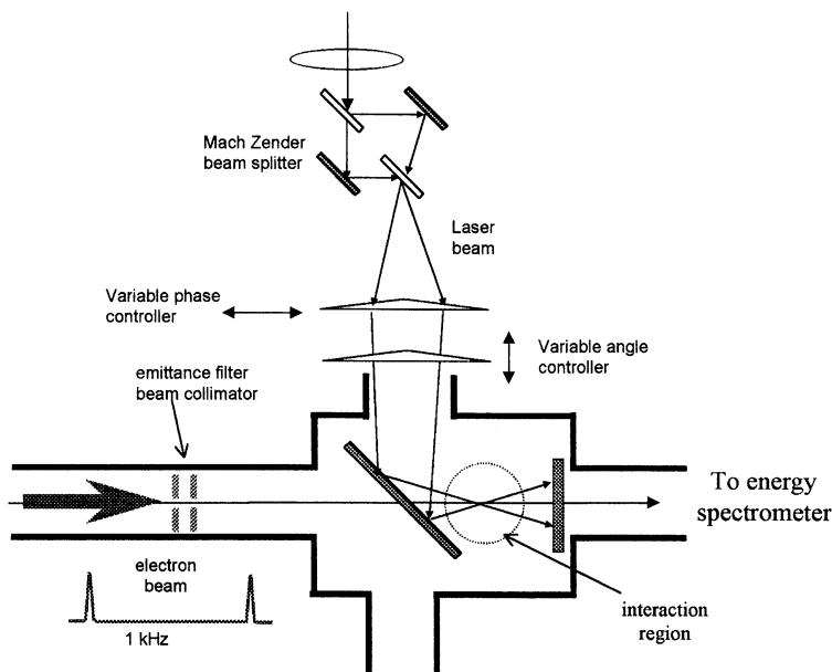
Fig. 5. The optical configuration at the interaction region. Each Ti : sapphire laser pulse is split into two identical ones at the Mach-Zehnder beam splitter. The prism, sliding in the horizontal direction, is to provide adjustments for the relative phase between the two pulses. The prism, sliding in the vertical direction, is to provide adjustments for the laser crossing angle. The emittance filter collimates electrons.
