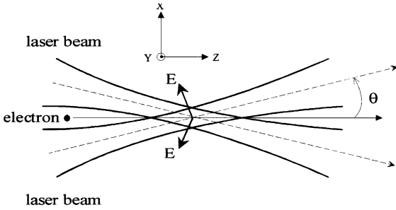
Fig. 1. The crossed-laser-beam electron acceleration scheme. The two linearly polarized laser beams are phased such that the transverse fields cancel and the longitudinal fields add along the electron axis. The inset defines the coordinate system used in this paper.
