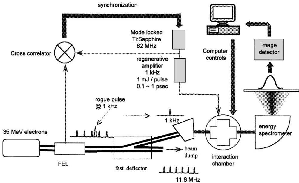
Fig. 4. Experimental setup for the LEAP experiment. The synchronization between the Ti:sapphire laser and the electron pulse is provided by the sum frequency generation of the FEL and the Ti:sapphire laser mixed in \text{AgGaSe}_2 . The rogue pulse at 1 kHz, unaffected by the FEL, is deflected into the interaction chamber by using a fast deflector.
