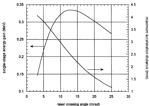
Fig. 3. Single-stage energy gain and the maximum acceleration distance versus the laser crossing angle, subject to the system parameters I_{\max} = 5 \text{ J cm}^{-2} , P_{\max} = 1 \text{ GW} , \theta_d = 4 \text{ mrad} , and \gamma = 70 . A large laser crossing angle causes more phase slippage, which reduces both the energy gain and the coherence length. On the other hand, a small crossing angle reduces acceleration field, but gives a better phase velocity matching.
