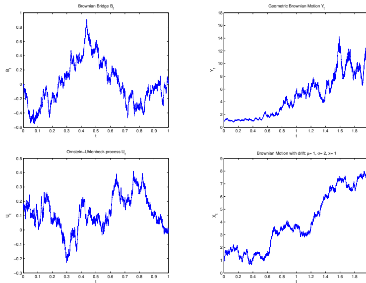
FIGURE 1. Illustration of sample paths for processes in Exercise 9.3.10.
