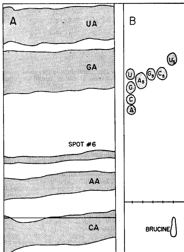
Fig. 1.—A, separation of 3.3 mg. of an alkaline hydrolysate of yeast ribonucleic acid by paper ionophoresis in 0.4 M ammonium formate buffer ( pH 3.3) at 80 milliamp. and 950 volts for 5 hours on Whatman No. 1 filter paper. CA, AA, GA and UA refer to cytidylic, adenylic, guanylic and uridylic acids. Spot 6 refers to substance 6 in fraction 2. B, separation of the 5'-nucleotides from their respective 3'-isomers by paper ionophoresis in 0.4 M sodium tetraborate buffer ( pH 9.2) at 30 millamp. and 850 volts for 2 hours on Whatman No. 1 filter paper. A, C, G and U refer to the respective 3'-nucleotides, while A 5 , G 5 , C 5 and U 5 refer to the respective 5'-nucleotides. U 5 was used as the brucine salt.
