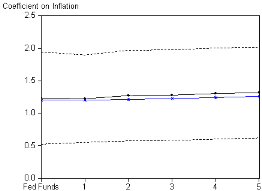
Fig. 6. The affine response coefficient (ARC) curve for inflation, derived from the model with both output and inflation and estimated over the period 1984Q1-2006Q4. The horizontal axis shows the maturity in years. The solid line with dots shows the estimated coefficients, the dashed lines show the 95% confidence intervals, and the solid line with stars shows the theoretical coefficients.
