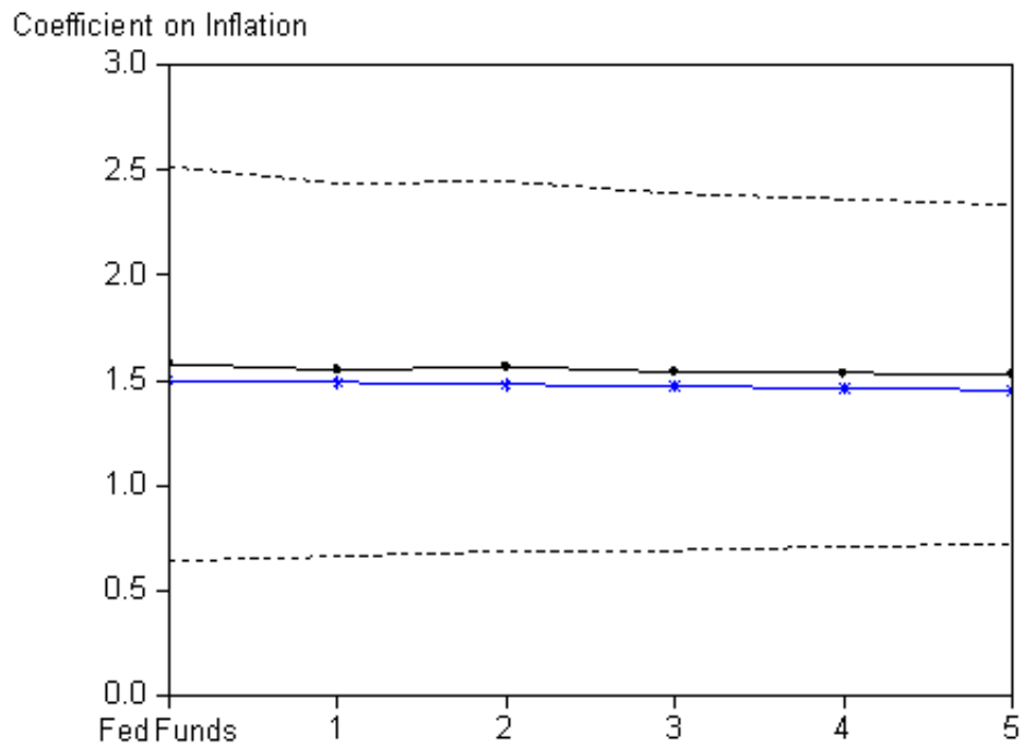
Fig. 2. The affine response coefficient (ARC) curve for inflation, derived from the model with inflation only and estimated over the period 1984Q1-2006Q4. The horizontal axis shows maturity in years. The solid line with dots shows the estimated coefficients, the dashed lines show the 95% confidence intervals, and the solid line with stars shows the theoretical coefficients.
