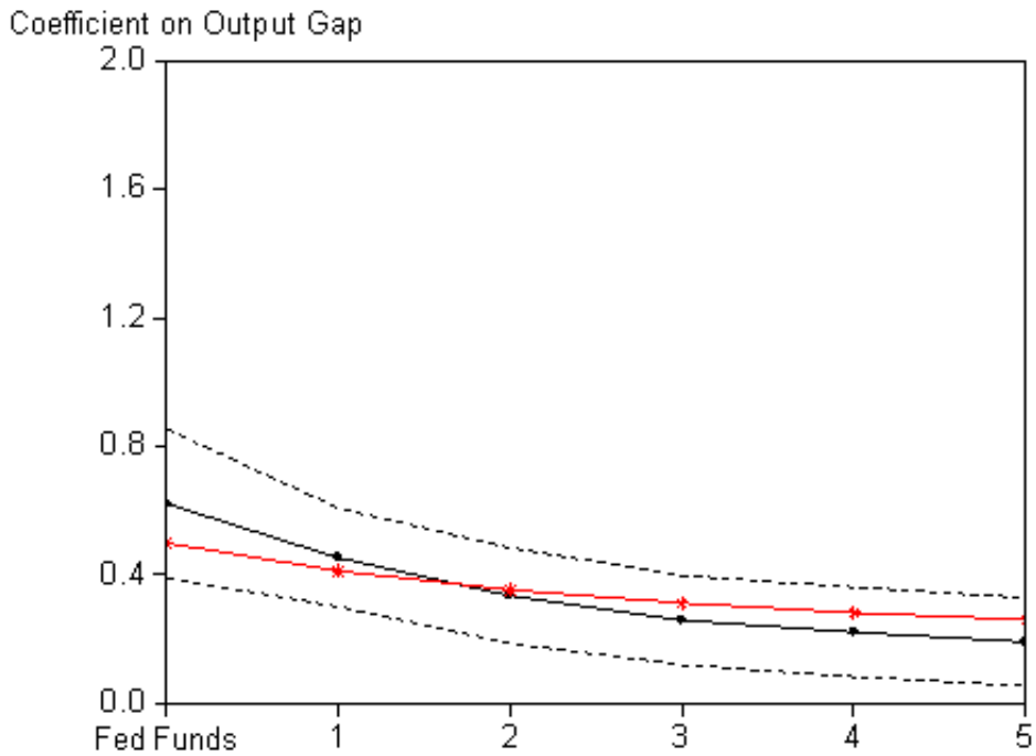
Fig. 3. The affine response coefficient (ARC) curve for output, derived from the model with both output and inflation and estimated over the period 1960Q1-1979Q4. The horizontal axis shows maturity in years. The solid line with dots shows the estimated coefficients, the dashed lines show the 95% confidence intervals, and the solid line with stars shows the theoretical coefficients.
