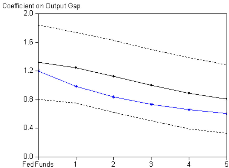
Fig. 4. The affine response coefficient (ARC) curve for output, derived from the model with both output and inflation and estimated over the period 1984Q1-2006Q4. The horizontal axis shows maturity in years. The solid line with dots shows the estimated coefficients, the dashed lines show the 95% confidence intervals, and the solid line with stars shows the theoretical coefficients.
