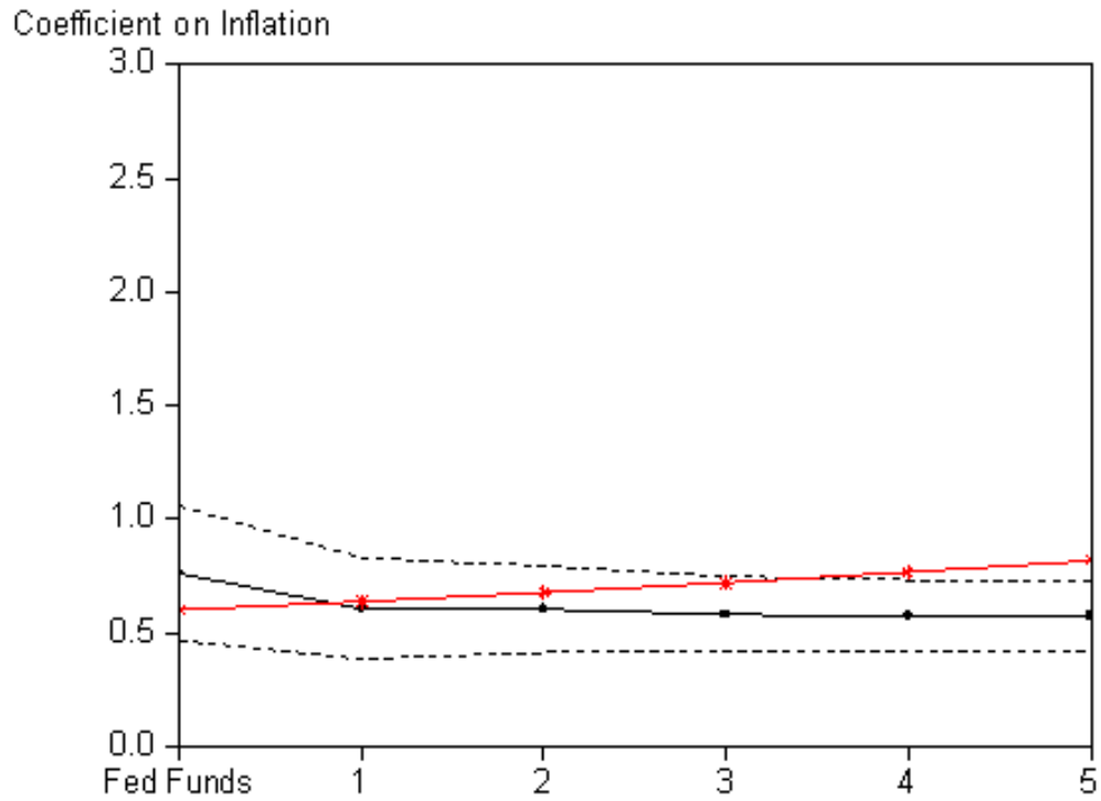
Fig. 1. The affine response coefficient (ARC) curve for inflation, derived from the model with inflation only and estimated over the period 1960Q1-1979Q4. The horizontal axis shows the maturity in years. The solid line with dots shows the estimated coefficients, the dashed lines show the 95% confidence intervals, and the solid line with stars shows the theoretical coefficients.
