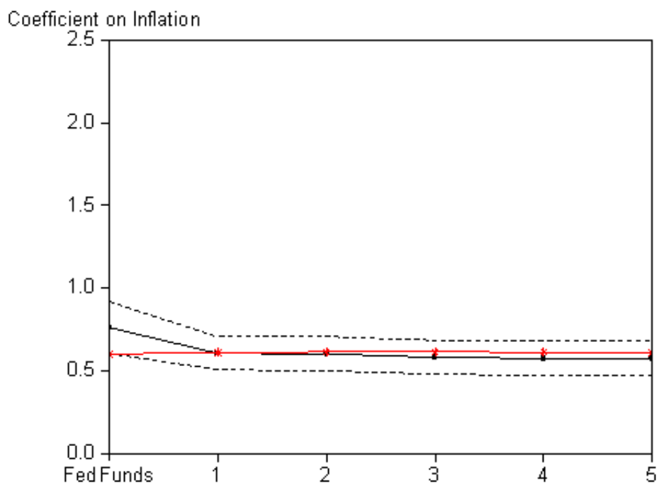
Fig. 5. The affine response coefficient (ARC) curve for inflation, derived from the model with both output and inflation and estimated over the period 1960Q1-1979Q4. The horizontal axis shows maturity in years. The solid line with dots shows the estimated coefficients, the dashed lines show the 95% confidence intervals, and the solid line with stars shows the theoretical coefficients.
