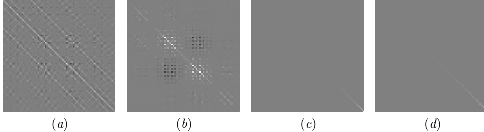
Figure 3. Covariance matrices for 128-dimensional SIFT (a) and 64-dimensional SURF (b) descriptors, and covariance matrices for transformed SIFT (c) and SURF (d) descriptors. Mid-gray represents zero.
