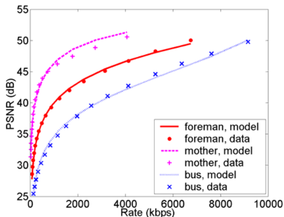
Fig. 2 Rate-PSNR performance of Foreman , Mother and Daughter and Bus CIF sequences, all encoded using H.264/AVC at 30 frames per second, with GOP length 15. The experimental data points are fitted with the model curve.
