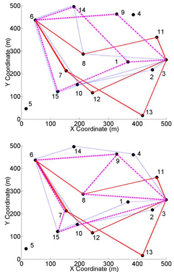
Fig. 6 Initial and final route selections of all three streams: Foreman in red solid line, Mother and Daughter in magenta dashed line and Bus in blue dotted line. Two routes for Mother and Daughter and three routes for Bus have changed over the iterations. For this instance, the \lambda in (8a) is chosen to be 0.1, and the rate increment is 100 kbps.
