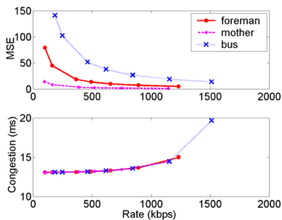
Fig. 3 Tradeoff between network congestion in terms of average link delay and video distortion in MSE resulting from the joint routing and rate allocation scheme, when streaming a single video sequence over the network.
