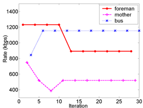
Fig. 7 Allocated rate for each stream over the iterations, corresponding to the same settings in Fig. 6 .
