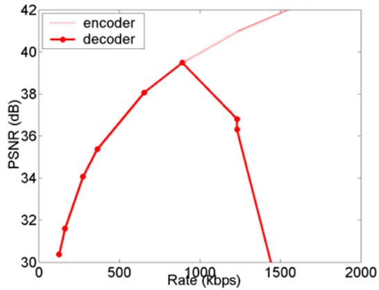
Fig. 4 Encoded and received video quality in PSNR versus allocated rate when streaming the Foreman sequence over the network using joint routing and rate allocation.
