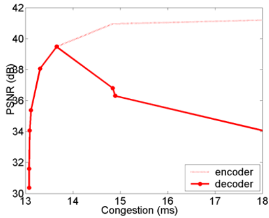
Fig. 5 Encoded and received video quality in PSNR versus network congestion in terms of average link delay when streaming the Foreman sequence over the network using joint routing and rate allocation.
