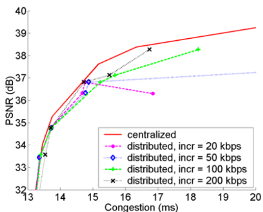
Fig. 8 Trade-off between overall network congestion in terms of average link delay and average video quality of all three video streams in PSNR, using the proposed distributed joint routing and rate allocation algorithm. The performance of the centralized solution is also plotted in solid lines for reference.
