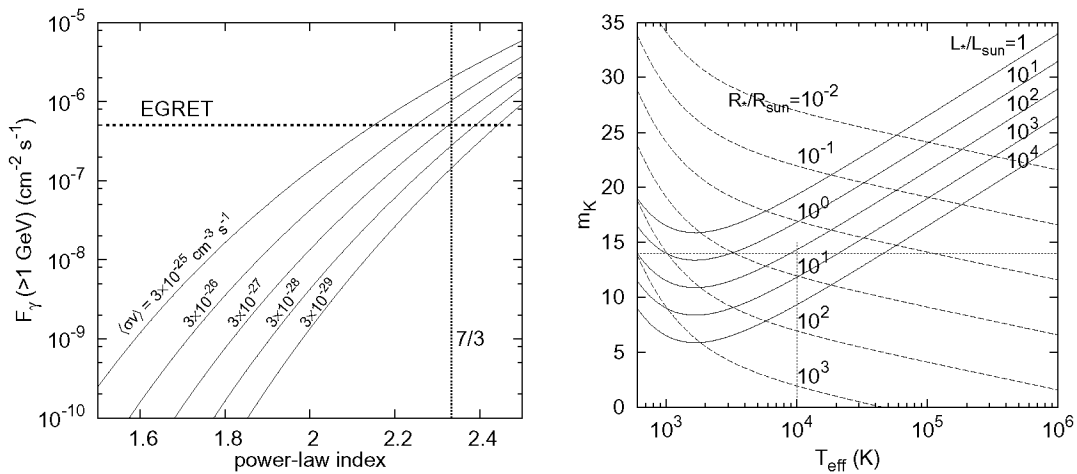
FIGURE 1. Left: \gamma -ray flux vs. the DM central spike power-law index. The lines are shown for a series of annihilation cross sections \langle\sigma v\rangle . Right: The visual K-band magnitude of DM burners at the GC without extinction vs. the effective surface temperature.
