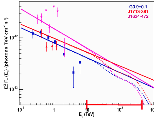
FIGURE 2. Attenuation on the ISRF for in-plane HESS sources. Line-styles: solid line, intrinsic spectrum; dashed line, attenuated spectrum. Data and locations of sources are summarised in [7]. The energy range of future experiments, such as TenTen [6] is indicated by the barred red line.
