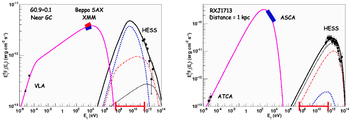
FIGURE 1. Left: Flux spectrum of G0.9+0.1. Line-styles: solid, total synchrotron and IC flux; dashed, optical IC; dash-dotted, infra-red IC; dotted, CMB IC. The GLAST energy range is indicated by the barred red line. Right: Flux spectrum of RXJ1713. Line-styles as for left panel. Data are summarised in [4].
