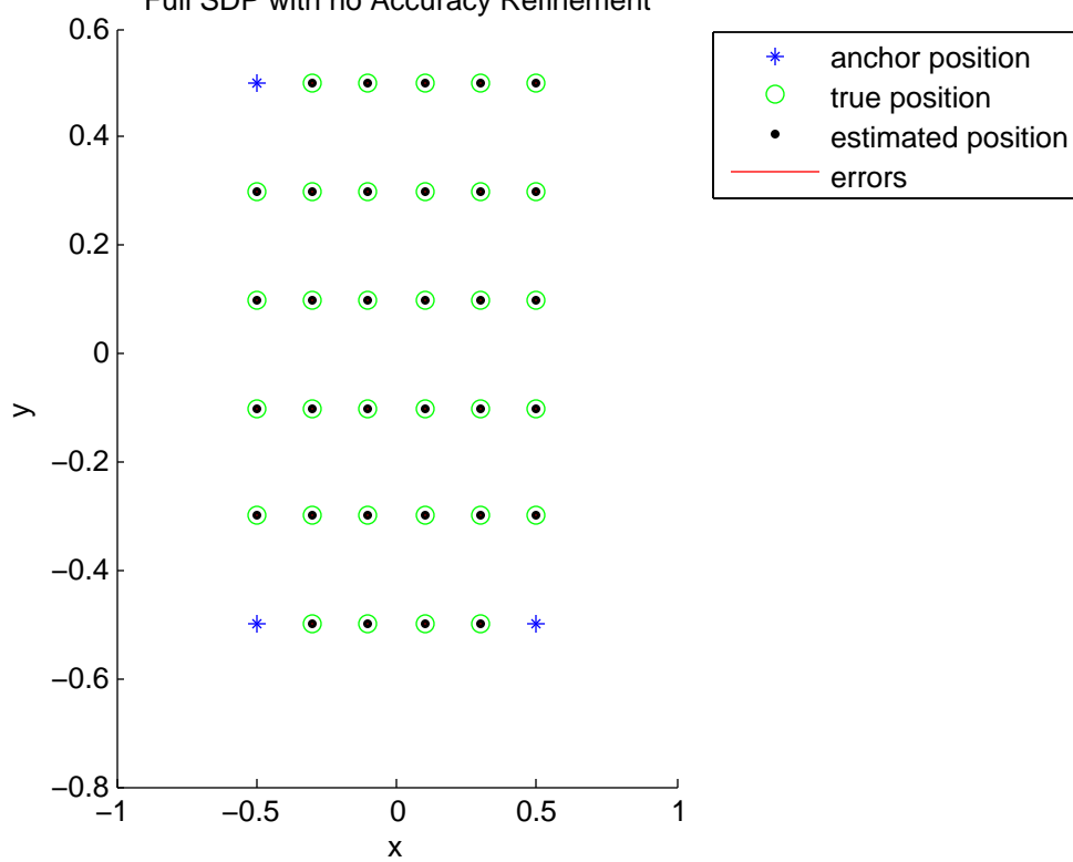
Full SDP with no Accuracy Refinement
