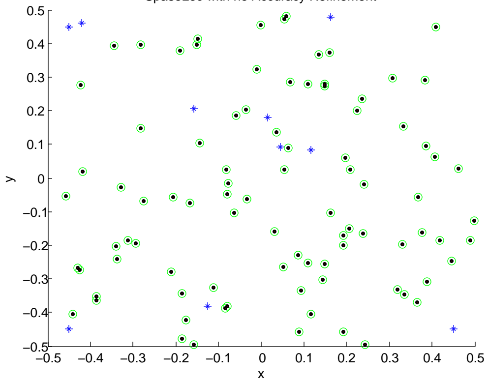
SpaseLoc with no Accuracy Refinement
