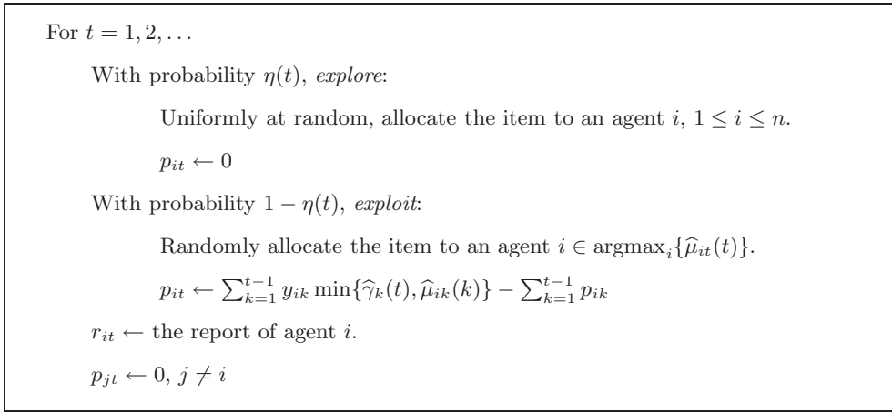
Figure 1: Mechanism \mathcal{M}
