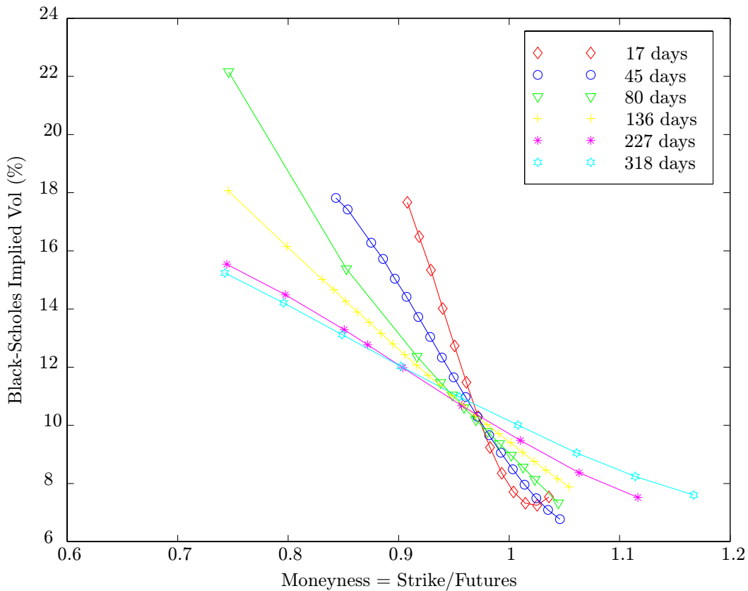
Figure1: “Smile curves” implied by SP500 Index options of 6 different times to expiration, from market data for November 2, 1993.
