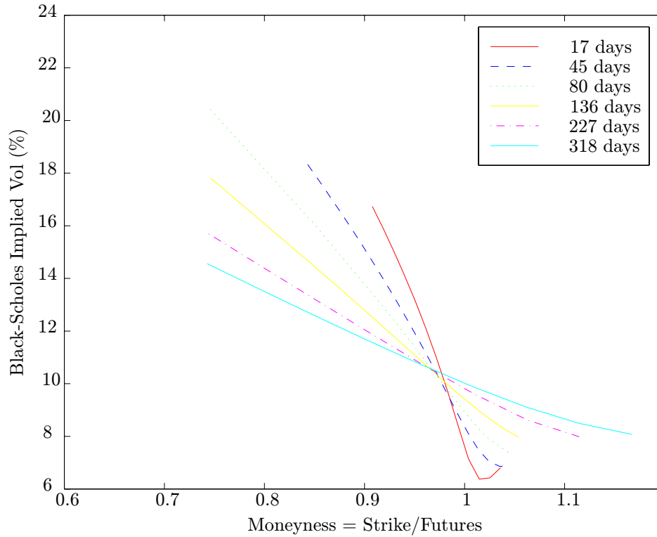
Figure2: “Smile curves” calculated for SP500 Index options of 6 different exercise dates, November 2, 1993, using the Heston Model.
