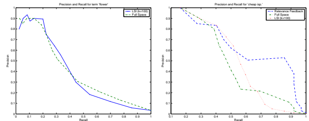
(a) Precision and Recall for “flower”. (b) Precision and Recall for “cheap isp”.
