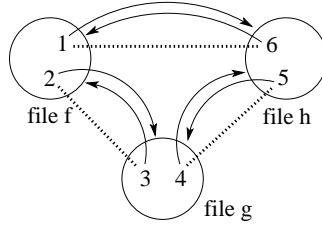
Fig. 2: Bilateral equilibrium for Ex.3. Peers \{1, 2\} have file f , peers \{3, 4\} have file g , and peers \{5, 6\} have file h . Solid arrows are drawn from a peer to its desired file, e.g., 1 and 4 want h . Heavy dotted lines are between peers bartering at the unique bilateral equilibrium.
