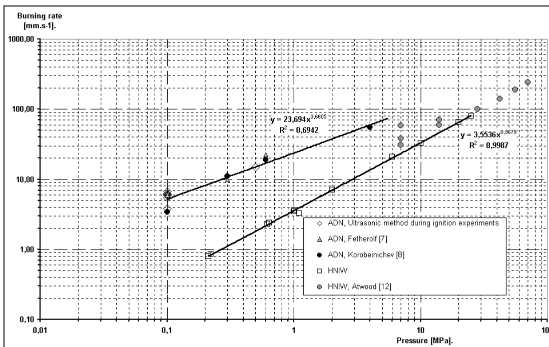
Figure 33: Burning Rate of HNIW (and ADN).
