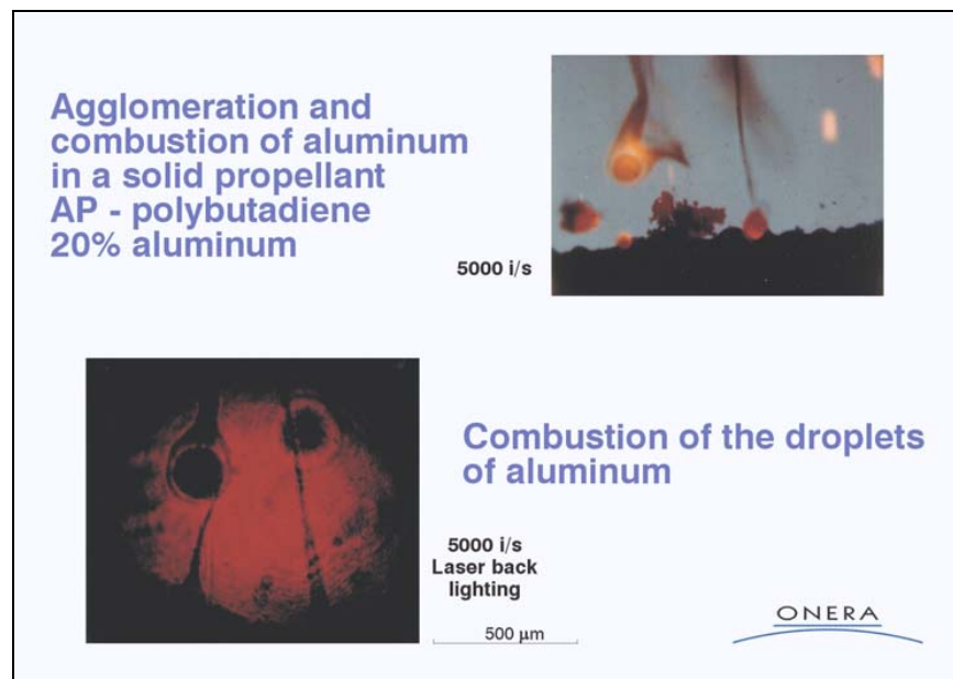
Figure 41: Aluminum Combustion.
