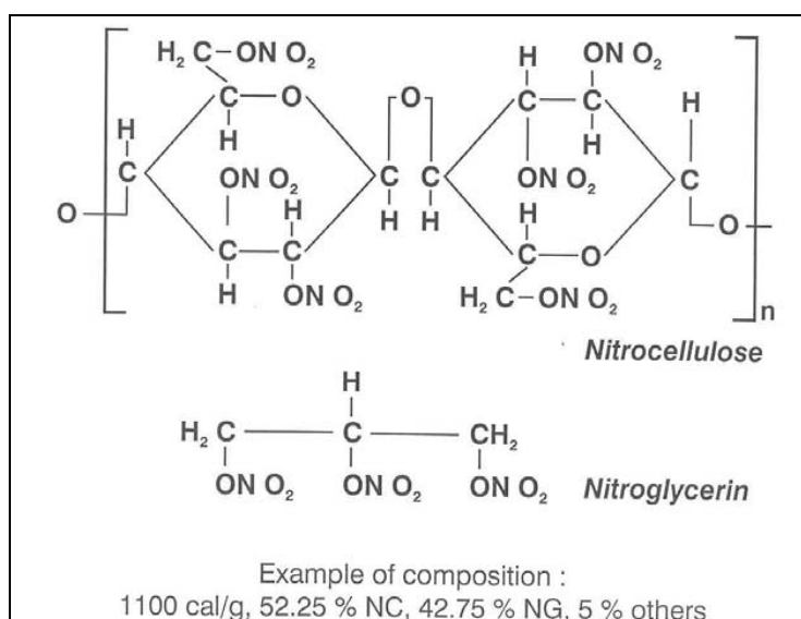
Figure 1: Components of Double Base Propellants.
