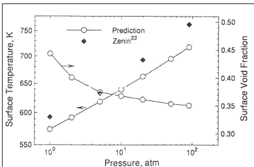
Figure 29: Conditions at the Surface of RDX [34].
