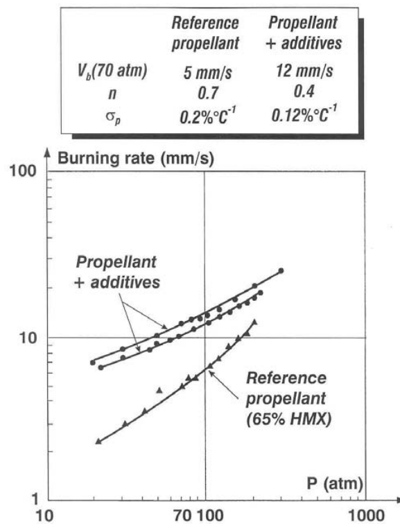
Figure 45: HMX – Active Binder Propellant with Additives.
