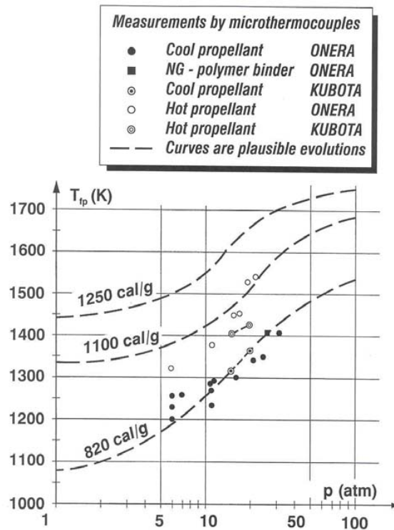
Figure 9: Primary Flame Temperature of Double Base Propellants.
