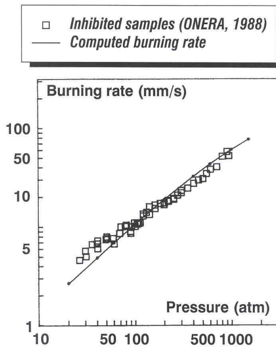
Figure 20: Burning Rate of Ammonium Perchlorate at High Pressures.
