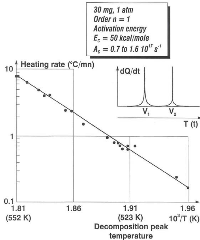
Figure 22: Differential Thermal Analysis of HMX Decomposition.
