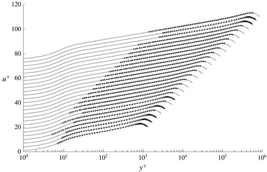
FIGURE 13. The PSP data and model profiles in this figure are identical to that shown in figure 7. The filled circles ( \bullet ) are determined from the model profile (3.5) and (3.13) with all parameters fixed at (\bar{k}, \bar{a}, \bar{m}, \bar{b}, \bar{n}) = (0.4092, 20.095, 1.621, 0.3195, 1.619) .
