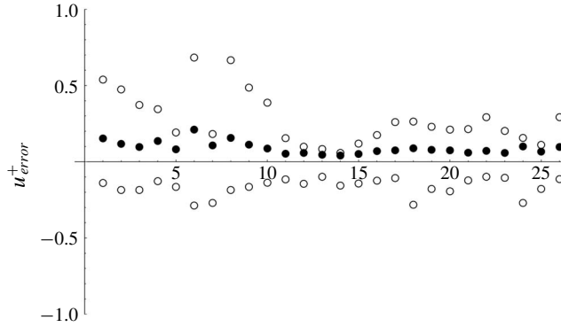
FIGURE 8. Errors in the fit of the universal velocity profile to the survey data. Filled circles, \bullet , are the root-mean-square error in u^+ between the model velocity profile (3.5) with wall-wake mixing length function (3.13) and the PSP velocity data. Maximum and minimum errors in u^+ are shown as open circles, \circ . Numbers on the horizontal axis refer to the PSP survey number.
