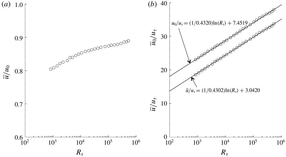
FIGURE 2. (a) PSP survey data for \bar{u}/u_0 and (b) wall shear stress in terms of \bar{u}/u_\tau and u_0/u_\tau versus R_\tau . Open circles in (b) ( \circ ) are data for PSP surveys 1 to 26. Least square log-linear fits to the data for PSP surveys 6 to 26 are shown as solid lines. Root-mean-square error in the upper solid line is 0.112 in units of u^+ . Root-mean-square error in the lower solid line is 0.0975.
