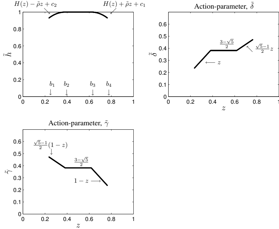
Fig. 7. A conjecture about the optimal solution based on the 20 th value iteration of the DP which is shown in Fig. 4 and on the questions given by Professor Cover. On the top-left, the conjectured differential value \hat{h}(z) is plotted for z \in [b_1, b_4] . On the top-right side and bottom-left, the conjectured policy (\tilde{\delta}(z), \tilde{\gamma}(z)) is plotted for z \in [b_1, b_4]
