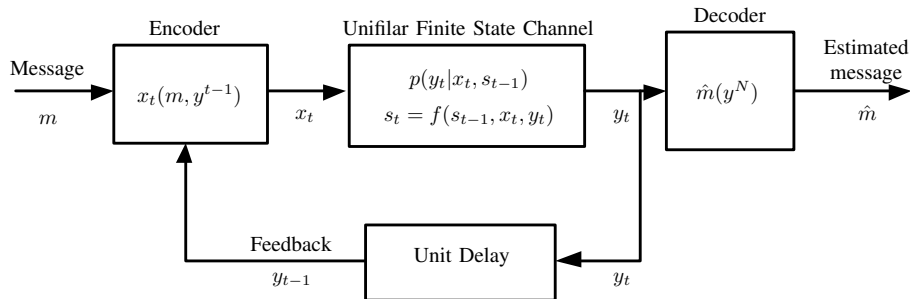
Fig. 2. Unifilar FSC with feedback
