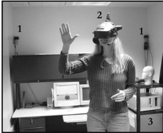
Figure 2. A depiction of our virtual environment system. The components are (1) position tracking cameras; (2) head-mounted display and orientation tracking sensor; and (3) image generator.
