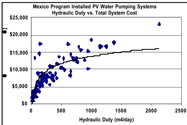
Figure 13. System costs based on hydraulic duty (m 4 ).
