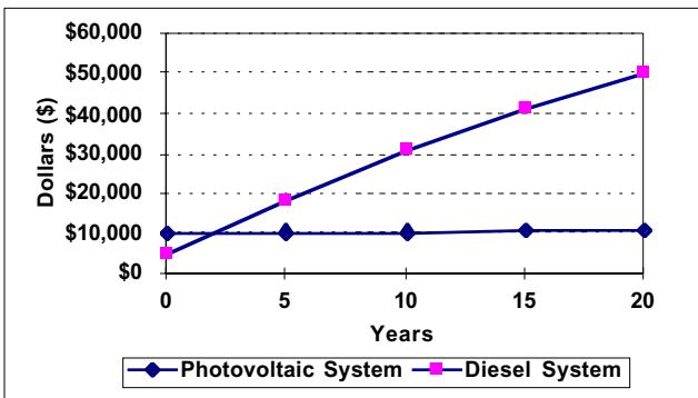
Figure 4. Life-cycle costs of Jeromin PV vs. diesel pump
