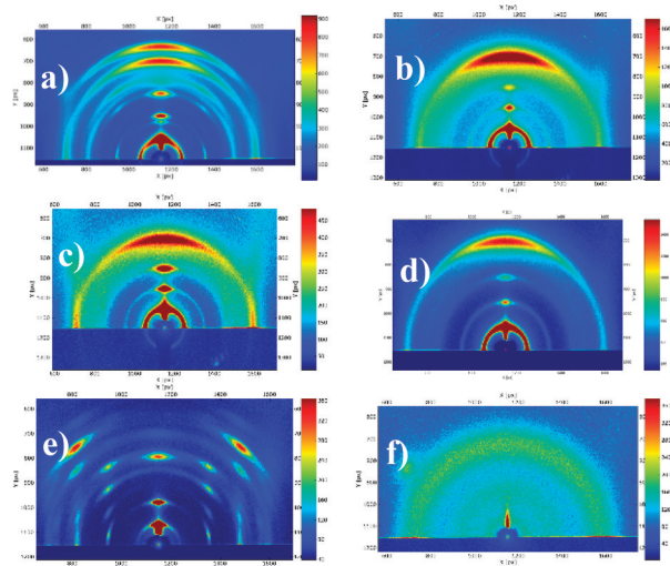
Figure 5. GI-XRD spectra of (a) P3HT:PI-BT spun from chlorobenzene (CB), (b) P3HT:NI-BT spun from chloroform (CF), (c) pure P3HT spun from CB, (d) pure P3HT spun from CF, (e) pure PI-BT spun from CB, and (f) pure NI-BT spun from CF. All samples were spun at 1500 rpm and thermally annealed at 110 °C for 10 min.
