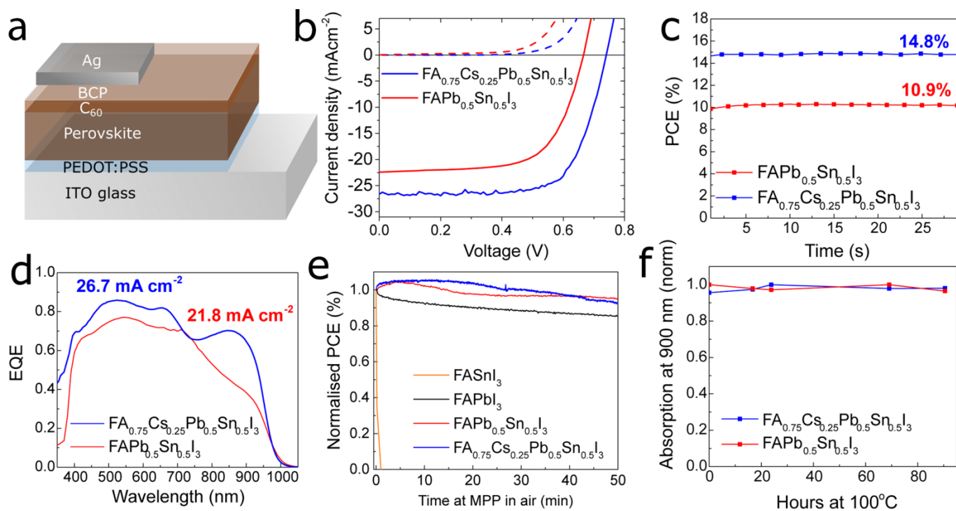
Fig. 2. Performance and stability of \text{FASn}_{0.5}\text{Pb}_{0.5}\text{I}_3 and \text{FA}_{0.75}\text{Cs}_{0.25}\text{Sn}_{0.5}\text{Pb}_{0.5}\text{I}_3 perovskite solar cells. (a) Schematic of the device architecture for narrow-gap single junction perovskite solar cells. (b) Current-voltage characteristics under AM1.5G illumination for the champion \text{FASn}_{0.5}\text{Pb}_{0.5}\text{I}_3 and \text{FA}_{0.75}\text{Cs}_{0.25}\text{Sn}_{0.5}\text{Pb}_{0.5}\text{I}_3 devices under illumination (solid lines) and in the dark (dotted lines), measured at 0.1V/s with no pre-biasing or light soaking. (c) Champion solar cells stabilized power output, measured via a maximum power point tracking algorithm. (d) External quantum efficiency for the champion devices of each material with the integrated current shown as an inset, providing a good match to the JV scan J_{\text{sc}} . (e) PCE as a function of time for three compositions of \text{FASn}_x\text{Pb}_{1-x}\text{I}_3 ( x=0, 0.5, 1 ) as well as \text{FA}_{0.75}\text{Cs}_{0.25}\text{Sn}_{0.5}\text{Pb}_{0.5}\text{I}_3 measured by holding the cell at maximum power point in air under AM1.5 illumination. (f) Thermal stability of \text{FASn}_{0.5}\text{Pb}_{0.5}\text{I}_3 and \text{FA}_{0.75}\text{Cs}_{0.25}\text{Sn}_{0.5}\text{Pb}_{0.5}\text{I}_3 films, quantified by heating the samples at 100°C and monitoring their absorption at 900 nm as a function of time.
