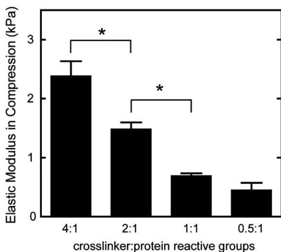
Fig. 2 Elastic modulus in compression of elastin-like hydrogels with varying crosslinking densities, reported as mean \pm SEM ( n = 4-6 ). Significant difference ( p < 0.05 ) as calculated by Tukey's post hoc test is denoted by *. Increasing the ratio of crosslinker to protein reactive groups increased the modulus of the elastin-like hydrogels.
