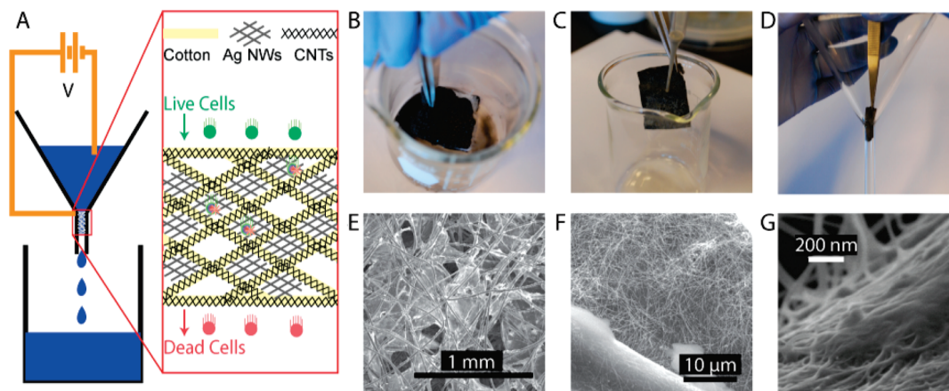
FIGURE 1. Schematic, fabrication, and structure of cotton, AgNW/CNT device. (A) Schematic of active membrane device proposed. (B) Treatment of cotton with carbon nanotubes (CNTs). (C) Treatment of device with silver nanowires (AgNWs). (D) Integration of treated cotton into funnel. (E) SEM image showing large scale structure of cotton fibers. (F) SEM image showing AgNWs. (G) SEM image showing CNTs on cotton fibers.
