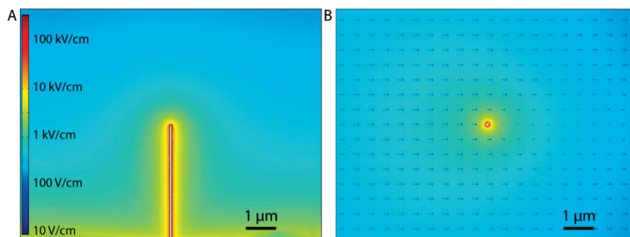
FIGURE 4. Simulation of e-field near NW surface in solution. log plot of the electric field near a NW in solution at experimental anodic conditions with (A) no flow and (B) a flow rate of 1 L/h, as calculated in a 2D geometry using finite element software solving the Nernst–Planck equations with electroneutrality. The scale for both panels is shown on the left side of panel A. The blue arrows in panel B show the direction and relative magnitude of convective \text{Na}^+ flux to illustrate the applied flow condition.
