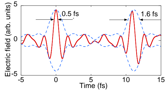
FIG. 4: The theoretically predicted electric field (thick line) and the corresponding field envelope (dashed line) that are synthesized by setting all of the Raman sideband phases to zero. The FWHM of the pulse envelope is 1.6 fs. The cosine pulse (left) is 0.5 fs long.
