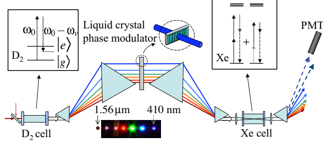
FIG. 1: Experimental set-up for temporal synthesis and characterization. Seven Raman sidebands are dispersed and their phases are independently varied by a liquid crystal modulator. The sidebands are recombined and focused into a target Xe cell. A solar-blind photomultiplier measures UV radiation that is generated in the Xe cell. The intensity of the generated UV wavelengths depends on the relative phases and amplitudes of the incident optical signal. (The 1.56\ \mu\text{m} sideband is not seen by the camera.)
