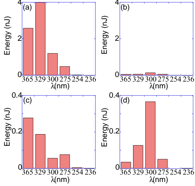
FIG. 2: Coherent control of the generated UV radiation. We plot the energies of the generated UV sidebands for different incident optical waveforms. Relative phases are adjusted to (a) maximize total UV generation, (b) minimize total UV generation, and (c), (d) invert the ratio of the energies at 365 nm and 300 nm. The energies of the incident Raman sidebands are approximately: 1.7 mJ at 1.56 \mu\text{m} ; 2.5 mJ at 1.064 \mu\text{m} ; 1.2 mJ at 807 nm; 2.5 mJ at 650 nm; 1.9 mJ at 544 nm; 0.8 mJ at 468 nm; and 0.5 mJ at 410 nm. [The energy at 254 nm in (d) was inadvertently not measured.]
