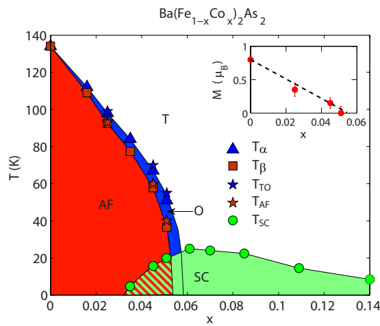
FIG. 2. (Color online) The phase diagram for \text{Ba}(\text{Fe}_{1-x}\text{Co}_x)_2\text{As}_2 determined from neutron scattering, heat capacity, and resistivity.
