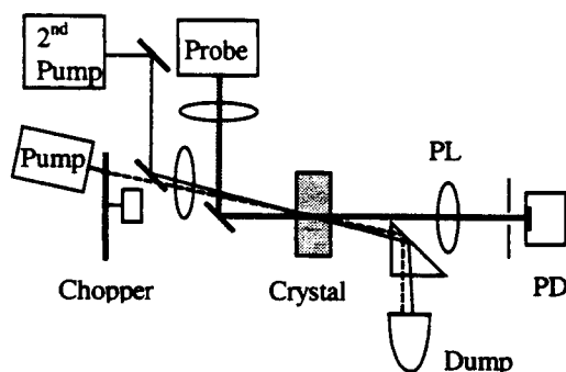
Figure 1. Crossed-beam setup for low absorption measurement. PL: projecting lens, PD: photodetector. Second pump is added whenever the influence of light with a different wavelength on absorption of the first pump is to be studied.
