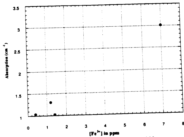
Figure 6: Effect of [\text{Fe}^{3+}] on absorption at 300 nm.
