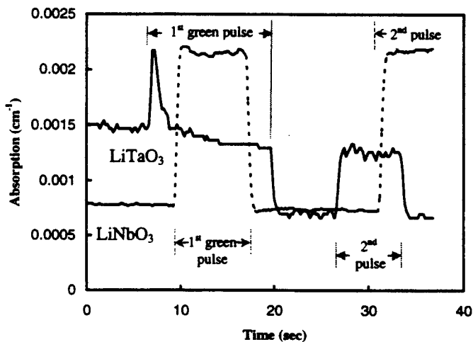
Figure 8. GRIIRA in LiTaO 3 #90 and oxygen-annealed LiNbO 3 : the response of absorption at 1064 nm for green light at a power density of 1.3 \text{ kW/cm}^2 which was applied as long pulses.
