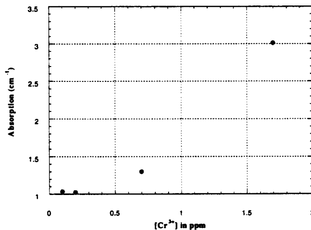
Figure 5: Effect of [\text{Cr}^{3+}] on absorption at 300 nm.
