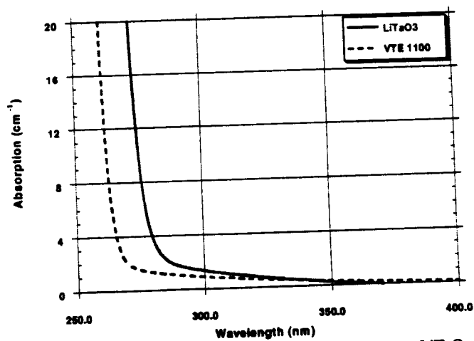
Figure 7: Effect on lithium enrichment on low-absorption \text{LiTaO}_3
