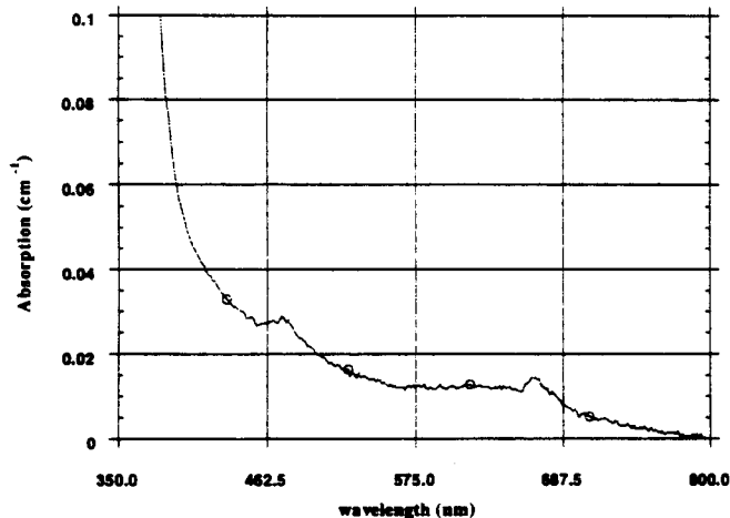
Figure 4: Absorption bands of \text{Cr}^{3+} in \text{LiTaO}_3 .
