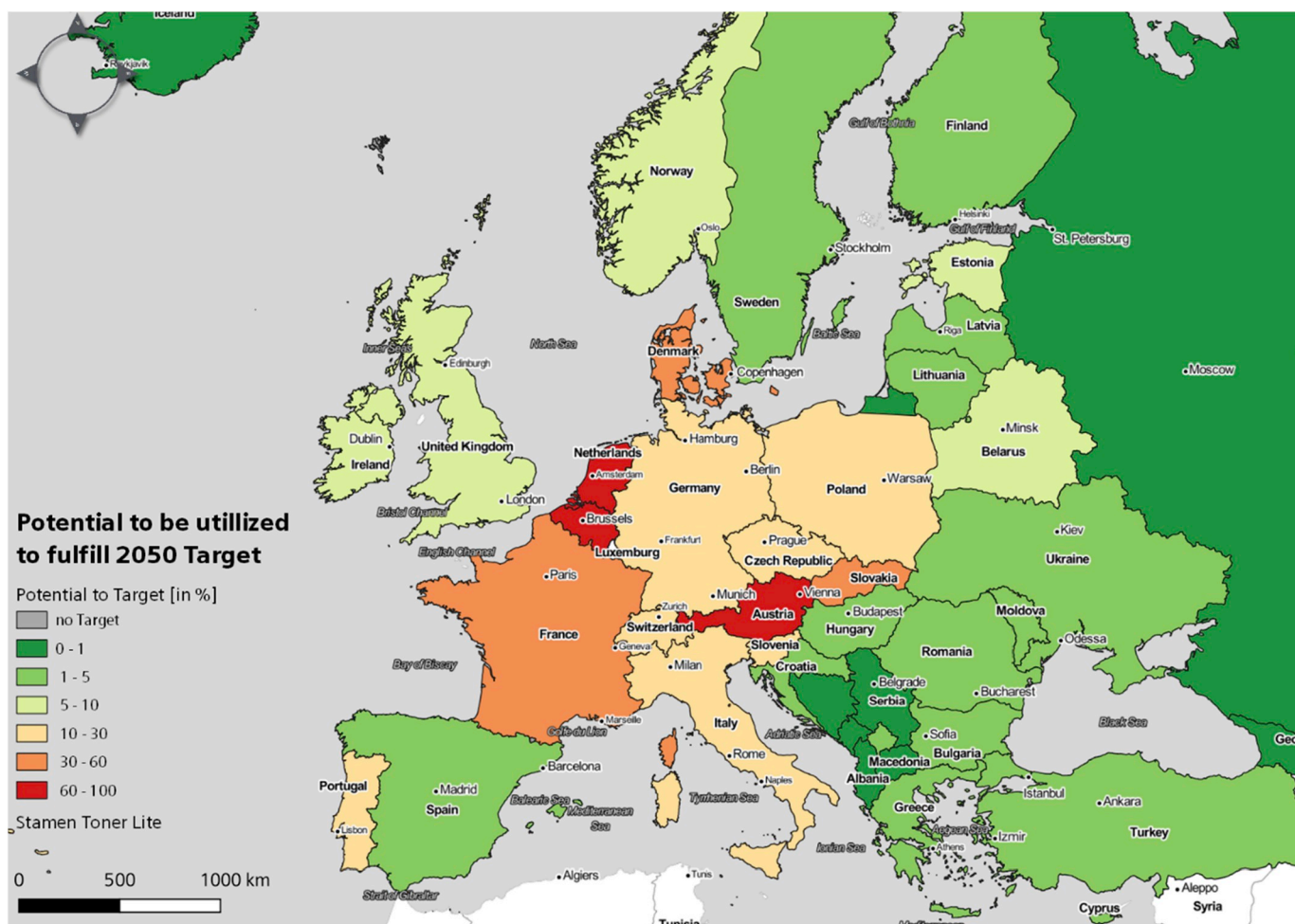
Fig. 6. The Difference between the potential nameplate capacity and the 2050 (Onshore) targets.
