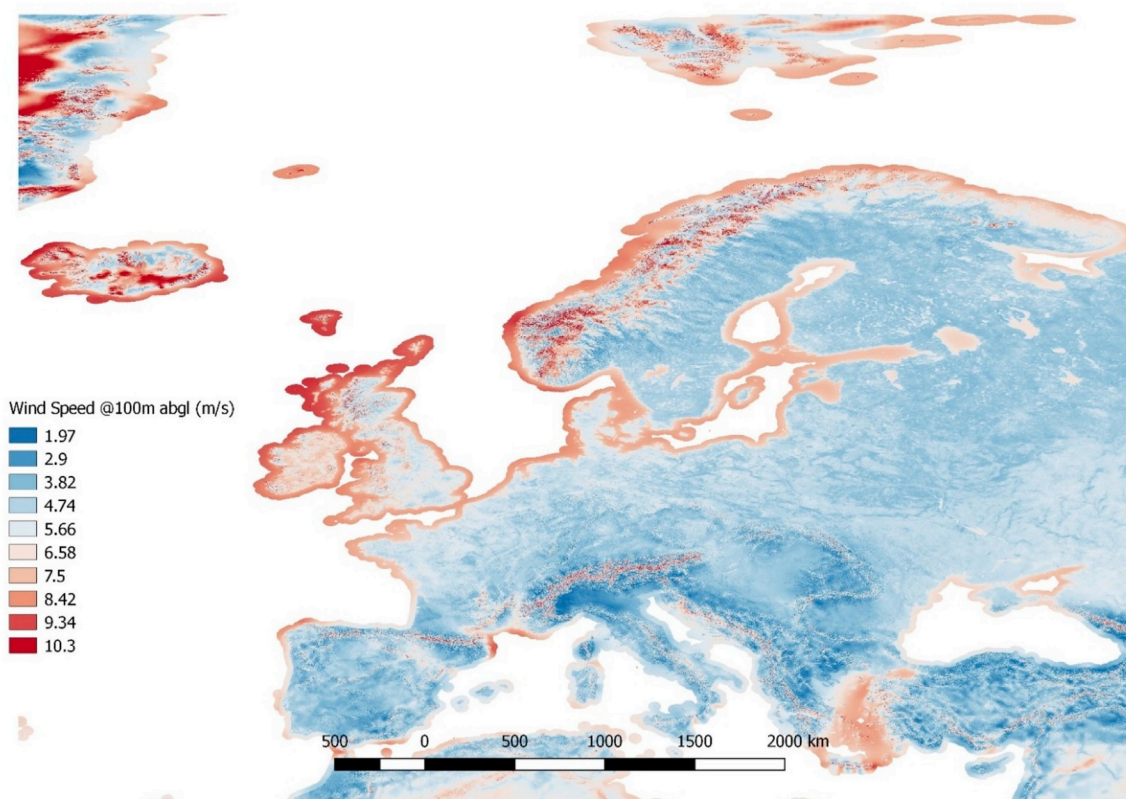
Fig. 3. Annual mean wind speeds at 100 m above ground level in Europe (Wind data from (The Global Wind Atlas, 2017)).
