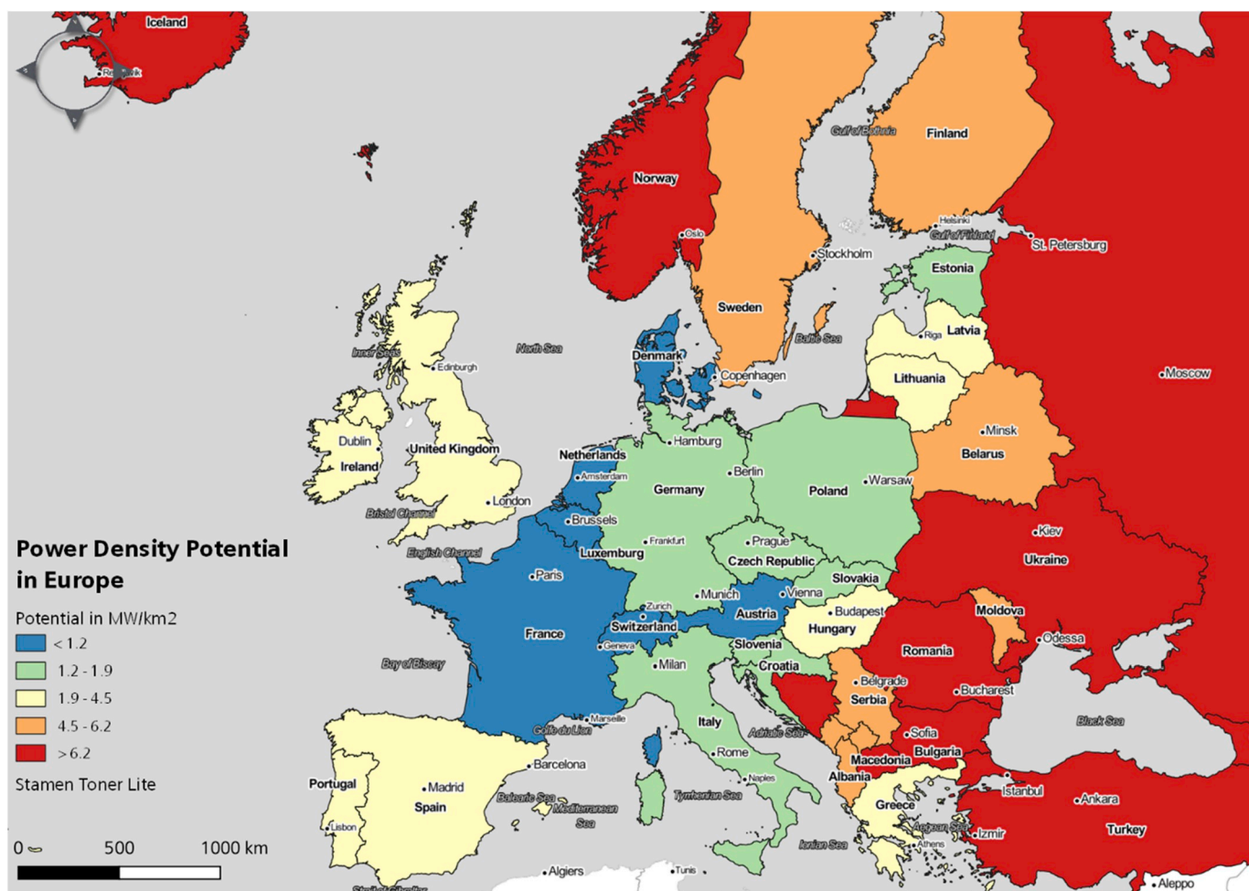
Fig. 5. The onshore potential for wind energy in Europe (MW/km 2 ).
