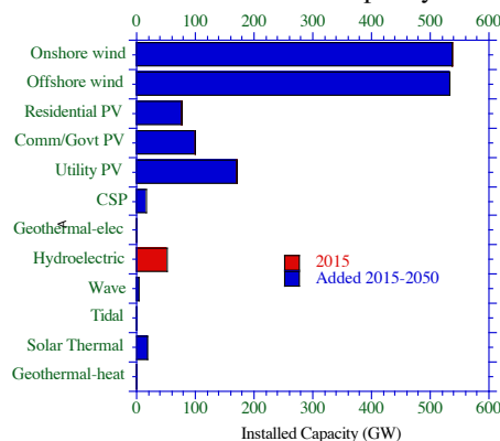
Figure 3. 2015 and proposed 2015-2050 additions of installed capacity of WWS generators for Russia-Georgia.
