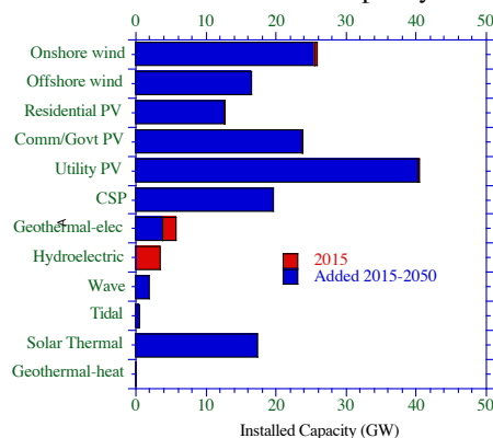
Figure 3. 2015 and proposed 2015-2050 additions of installed capacity of WWS generators for the Philippines.
