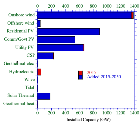
Figure 3. 2015 and proposed 2015-2050 additions of installed capacity of WWS generators for India-Nepal-Sri Lanka.
