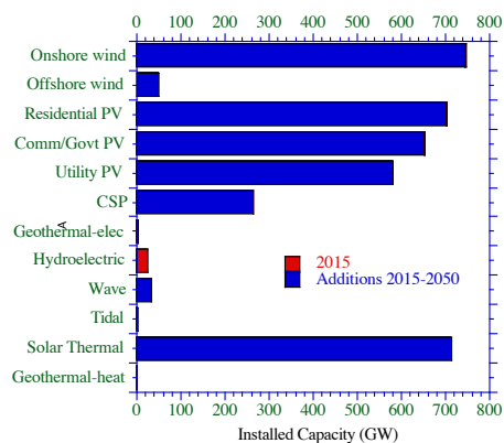
Figure 3. 2015 and proposed 2015-2050 additions of installed capacity of WWS generators for 27 countries in Africa.
