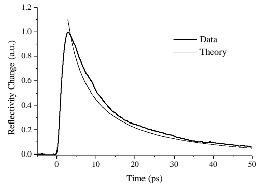
Fig 2: Reflectivity data and theoretical fit to 6 ps diffusive conduction time constant. Gate opens and closes with a 9.3 ps FWHM creating a 10% change from initial reflectivity.
