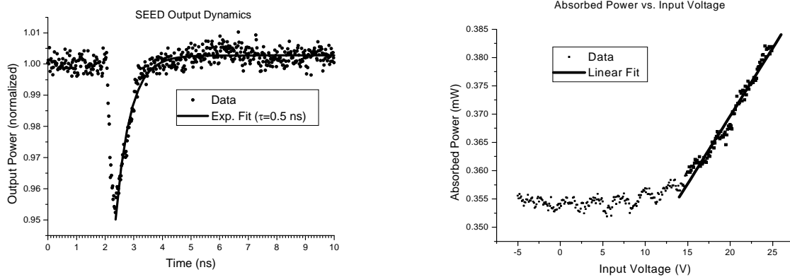
Fig. 2. (a) Modulated output power of SEED as a function of time. The power drops sharply after the sampling optical pulse hits the MSM switch, then recovers with a fitted exponential time constant of 0.5 ns as the SEED discharges itself through the absorption process. This is in good agreement with the predicted time constant of approximately 0.4 ns. (b) Absorbed power versus input voltage. The absorbed power (and hence output power) is linearly proportional to the input voltage when the input is large enough to keep the SEED out of forward bias.
