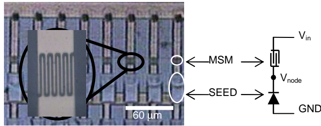
Fig. 1. Micrograph and schematic of the MSM photoconductive switch and SEED modulator in series. In normal operation, a short optical pulse triggers the sampling of an input signal V_{in} onto V_{node} . The SEED modulates a CW beam, producing an output beam whose integrated power over a sampling period is a linear representation of the sampled voltage.
