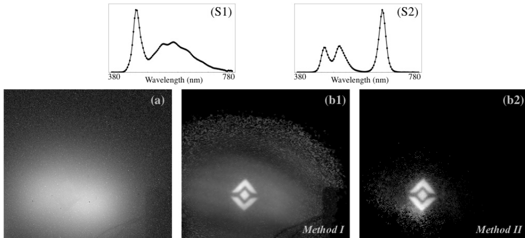
Figure 2: Detection of a narrowband tag: (a) the hidden tag S2 has the same color and intensity as the surrounding surface S1. (b1, b2) light emitted from the tag is detected because it exhibits a higher coherence length.
