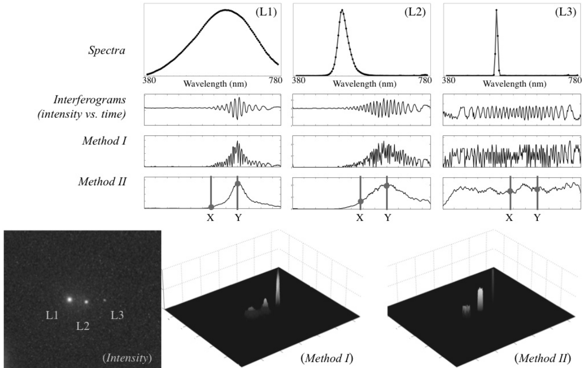
Figure 1: Sensing intensity and coherence length using Method I and II for three different light sources (L1, L2, L3); black floor represents image plane and height indicates coherence length.
