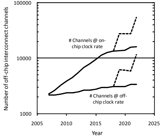
Fig. 4. Number of channels required to support the ITRS off-chip interconnect bandwidth [40], presuming either the ITRS off-chip or on-chip clock rate respectively for those channels (solid lines). The dashed lines show the corresponding numbers if the number of bytes/FLOP is maintained in the later years.
