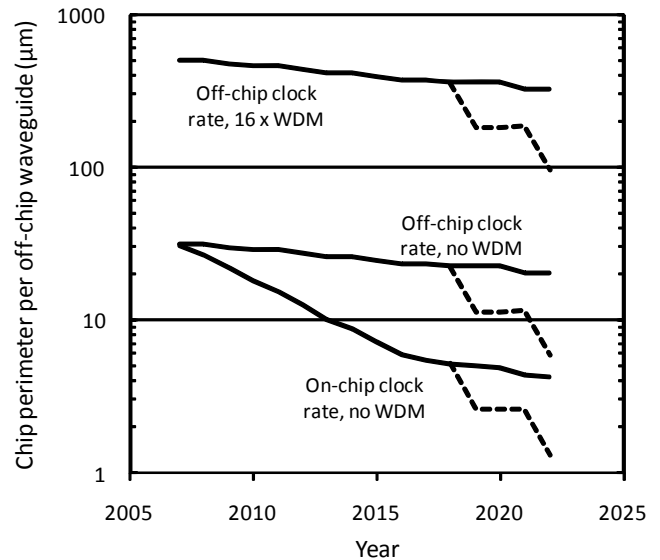
Fig. 5. Available width per waveguide channel for waveguides brought off the chip edge. Upper lines – channels running at the off-chip ITRS clock rate, and with 16 WDM channels on each waveguide. Middle lines – channels running at the off-chip ITRS clock rate, with one channel per waveguide. Lower lines – channels running at the on-chip ITRS clock rate, with one channel per waveguide. The solid lines presume the bandwidths from the product of the off-chip clock rate and the number of signal pins from the ITRS roadmap [40]. The dashed lines presume that the number of bytes of off-chip interconnect per floating point operation (i.e., the number of bytes/FLOP) is to be maintained in the later years.
