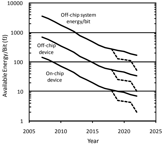
Fig. 3. The available energies per bit for interconnects, including the total available system energy per bit for off-chip interconnects (top lines), the energy per bit available for the optical output devices to drive the off-chip interconnect (middle lines), presumed to be 20% of the system energy per bit, and the energy per bit available for optical output devices to drive the on-chip global interconnects (bottom lines). The global on-chip interconnects are presumed to have 5 times the off-chip bandwidth. The solid lines presume the bandwidths from the product of the off-chip clock rate and the number of signal pins from the ITRS roadmap [40]. The dashed lines presume that the number of bytes of off-chip interconnect per floating point operation (i.e., the number of bytes/FLOP) is to be maintained in the later years. The middle lines also happen to represent the system energy/bit for on-chip global interconnects because we take that energy also to be five times the device energy for on-chip global interconnects.
