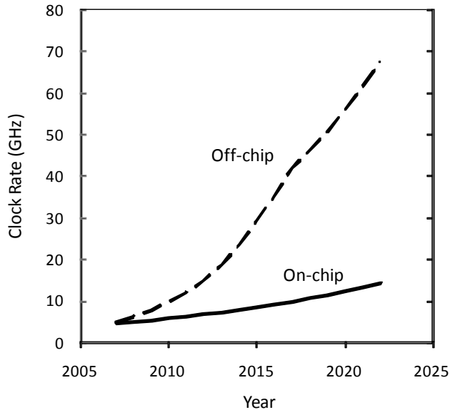
Fig. 2. Projected on-chip clock rate and the projected off-chip rate required to drive the chip input and output, according to the ITRS roadmap [40]
