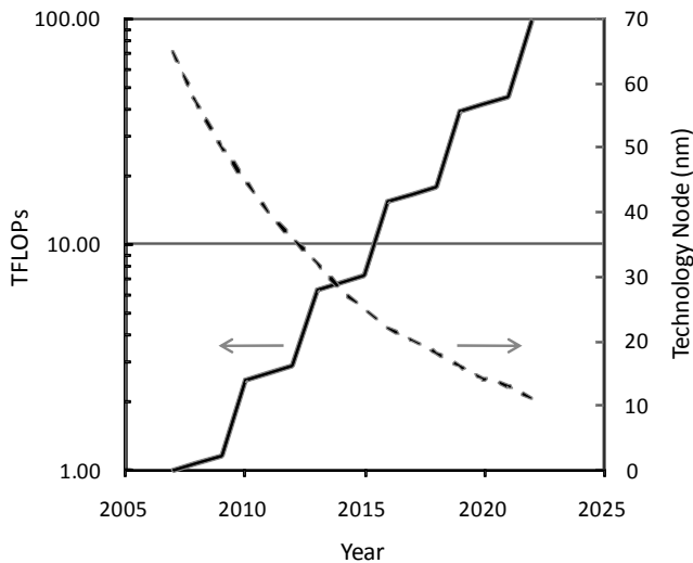
Fig. 1. The technology node (a characteristic feature size) for silicon CMOS, and the projected number of floating point operations (FLOPs) (units TFLOPs = 10^{12} FLOPs), scaling by the product of the number of transistors times the on-chip clock rate [40], from a presumed 1 TFLOP in 2007 ([56]).
