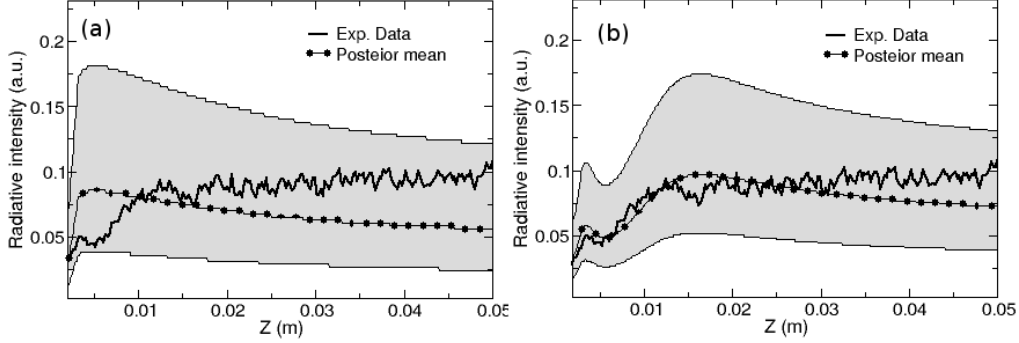
FIGURE 5. Predicted radiation intensity integrated over 772–782 [nm] (a) one-temperature model and (b) two-temperature model. For both cases, the scenario is the same as shot #47 reported in Table 1. The gray region denotes the 95% confidence interval (CI).
