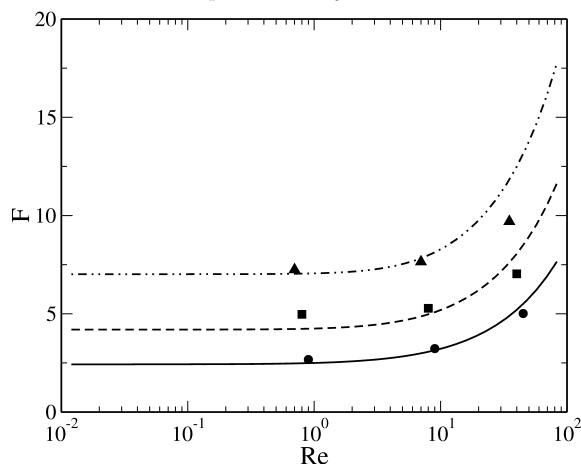
FIGURE 4. Non-dimensional drag force as function of the particle Reynolds number for random arrangements of spheres. Comparison between the model of Beetstra et al. (2007) (lines) and present work (symbols). \varepsilon = 0.9 (circles), 0.8 (squares), and 0.7 (triangles).
