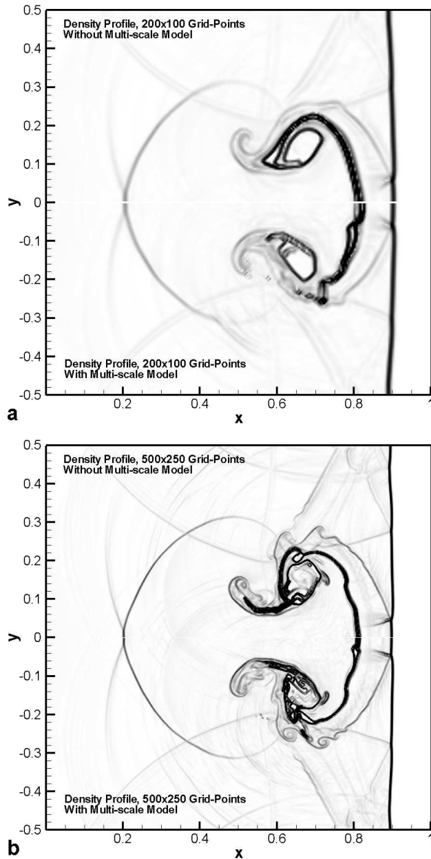
FIGURE 3. Comparison of the results of the shock-bubble interaction problem at time t = 0.2 : Schlieren-type images (mirrored images from symmetric axes are results with a multi-scale model) of density for (a) \Delta = 5 \times 10^{-3} , and (b) \Delta = 2 \times 10^{-3} .
