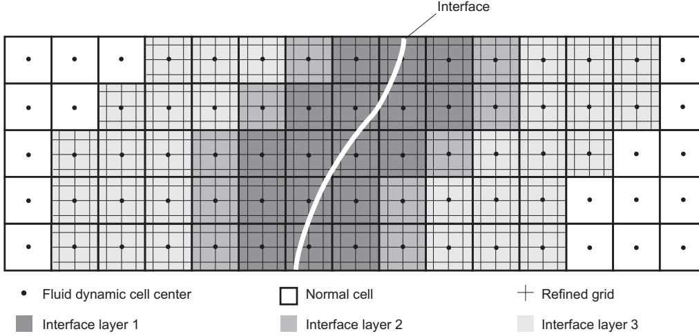
FIGURE 1. Schematic of the two-scale grid system with a refinement ratio of 3.
