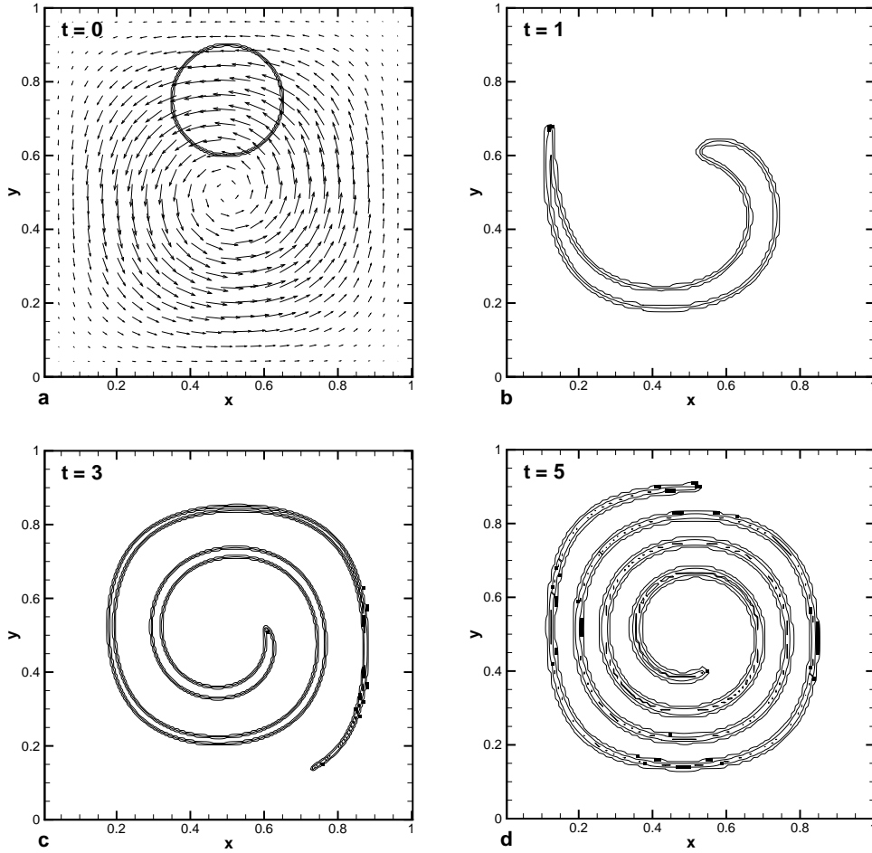
FIGURE 2. Results of interface deformation in the single vortex flow using a two-scale grid system ( \Delta = 0.01 , r = 3 , volume fraction contours of \alpha = 0.05, 0.5 and 0.95 obtained from level sets on the coarse grid): (a) initial interface location and velocity field, (b), (c) and (d) cells with unresolved interface (black squares) at time t = 1, 3, 5 .
