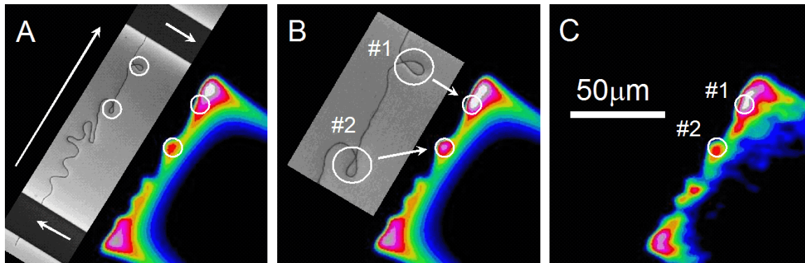
Figure 1: Scanning SQUID microscopy of nanotube loops. (A) Modeled SQUID image under the assumption of 100% current tunneling through the nanotube-nanotube junctions. An SEM image of the entire device is shown as an inset. (B) Modeled SQUID image under the assumption of 100% current flowing through the loops. A magnified view of the two loops is shown as an inset. (C) Experimental SQUID image from the CNTFET. The 1kHz, AC source-drain currents detected by the SQUID were between 1 and 2 microA, and the devices operated as p-type devices with a negative V_d and negative time varying V_g 's.
