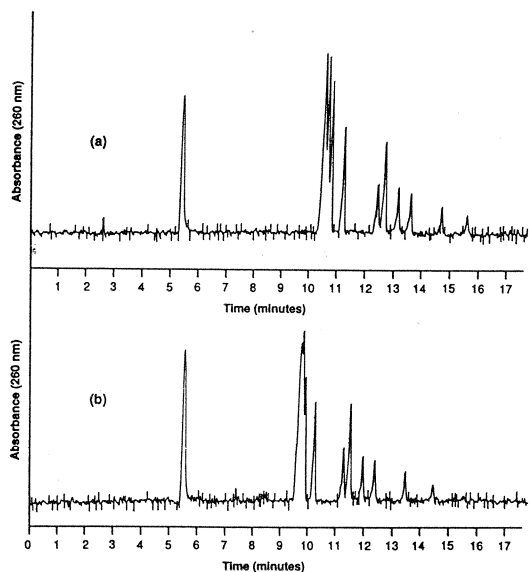
Fig. 9. Capillary electrophoresis of \Phi X174/ Hae III restriction fragments ranging in size from 72 to 1353 bp in (a) 0.95% (w/w) M_n 35 900 HEC, and (b) 1.35% (w/w) M_n 35 900 HEC, both in 89 mM Tris-89 mM boric acid-5 mM EDTA. Reading from left to right (not including the first peak, which is a neutral marker), the species are 1353, 1078, 872, 603, 310, 281 + 271, 234, 194, 118, and 72 bp in length, respectively. Conditions: field strength 221.4 V/cm; current (a) 8.8 \mu A, (b) 9.3 \mu A; UV detection at 260 nm; capillary dimensions, 50 cm total length (35 cm to detector) \times 51 \mu m I.D.; temperature, 30 \pm 0.1^\circ\text{C} . R.S.D. of absolute electrophoretic mobilities: (a) 1.16%, n = 5 ; and (b) 0.93%, n = 7 .
