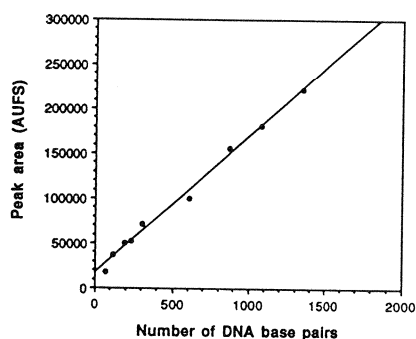
Fig. 8. A representative plot of UV absorbance peak area vs. number of DNA base pairs. This particular plot was obtained for electrophoresis at 220 V/cm of \Phi X174/ Hae III restriction fragments in a buffer containing 0.22% (w/w) M_n 105 000 HEC.
