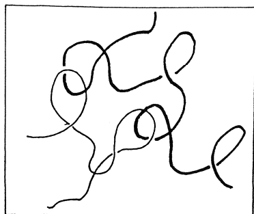
Fig. 2. Long-range entanglement coupling between two polymers. Since the presence of bulky side-groups, like the ethylene oxide group of HEC, does not inhibit the onset of entanglement coupling in solutions of cellulosic polymers, it seems likely that these interactions involve long-range looping rather than short-range kinking or knotting [12].
