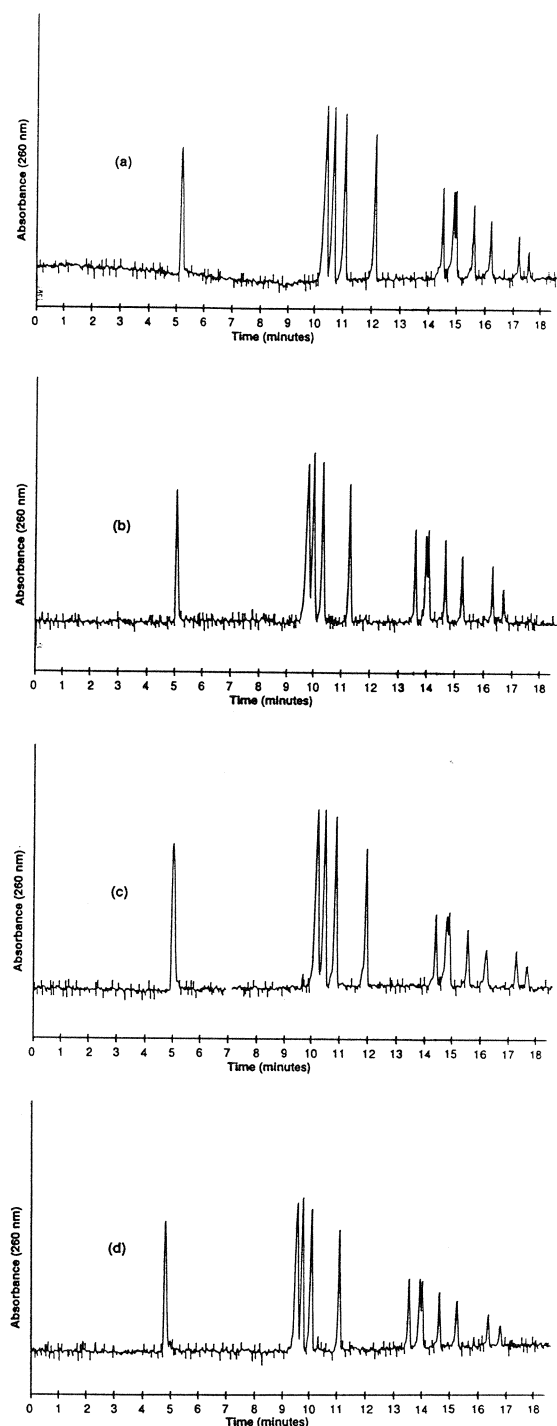
Fig. 10. Capillary electrophoresis of \Phi X174/ Hae III restriction fragments ranging in size from 72 to 1353 bp in (a) 0.225% (w/w) M_n 105 000 HEC, (b) 0.225% (w/w) M_n 160 000 HEC, (c) 0.22% (w/w) M_n 306 000 HEC, (d) 0.225% (w/w) M_n 438 800 HEC, all in 89 mM Tris-89 mM boric acid-5 mM EDTA. Reading from left to right (not including
