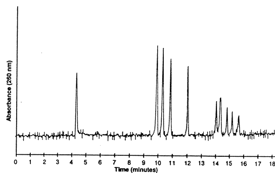
Fig. 11. Capillary electrophoresis of \Phi X174/HaeIII restriction fragments ranging in size from 72 to 1353 bp in 0.12\% (w/w) M_n 438\,800 HEC, 89 mM Tris- 89 mM boric acid- 5 mM EDTA. Reading from left to right (not including the first peak, which is a marker), the species are 1353 , 1078 , 872 , 603 , 310 , 281 + 271 , 234 , 194 , 118 + 72 bp in length, respectively. Conditions: field strength 221.4 V/cm; current 7.1 \mu A; UV detection at 260 nm; capillary dimensions, 50 cm total length ( 35 cm to detector) \times 51 \mu m I.D.; temperature, 30 \pm 0.1^\circ C. R.S.D. of absolute electrophoretic mobilities: 0.54\% , n = 3 .
