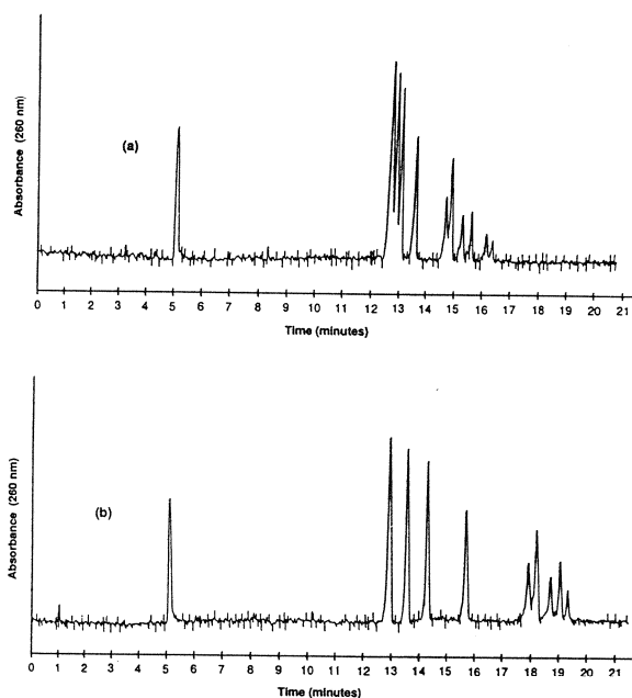
Fig. 7. Capillary electrophoresis of eleven \Phi X174/HaeIII restriction fragments ranging in size from 72 to 1353 bp in (a) 0.35% (w/w) M_n 27000 HEC, and (b) 0.09% (w/w) M_n 105000 HEC, both in 89 mM Tris-89 mM boric acid-5 mM EDTA. Reading from left to right (not including the first peak, which is a neutral marker), the species are (a) 1353, 1078, 872, 603, 310, 281 + 271, 234, 194, 118, and 72 bp in length, and (b) 1353, 1078, 872, 603, 310, 281 + 271, 234, 194 + 118, 72 bp in length, respectively. Conditions: field strength 221.4 V/cm; current (a) 7.2 \mu A , (b) 7.1 \mu A ; UV detection at 260 nm; capillary dimensions, 50 cm total length (35 cm to detector) \times 51 \mu m I.D.; temperature, 30 \pm 0.1^\circ C . R.S.D. of absolute electrophoretic mobilities: (a) 0.21%, n = 5 ; and (b) 0.37%, n = 6 .
