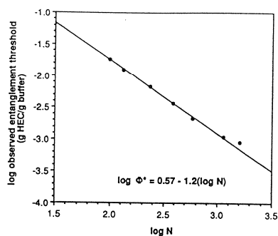
Fig. 5. A plot of the logarithm of the entanglement threshold (g HEC/g buffer) vs. the logarithm of the number of HEC monomers in the chain, showing that \Phi^* scales as N^{-1.2} .
