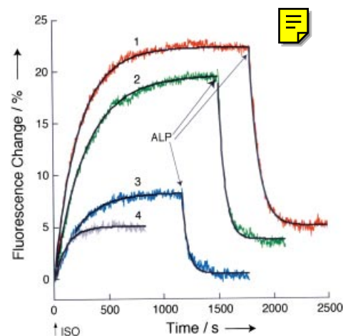
Figure 2. Activation of TMR-5- \beta_2 AR (35 nm) monitored in a standard fluorometer. 1) Fluorescence emission was recorded over time after addition of ISO, EPI, or SAL (100 \mu M; time = 0 sec). Typical fluorescence traces are shown after exposure with ISO (1), EPI (2), and SAL (3). The fluorescence intensity increased by 23, 19, and 8%, with t_{1/2} values of 177 \pm 1 , 167 \pm 1 , and 144 \pm 2 s, respectively. After equilibrium was reached, ALP (10 \mu M) was added, which induced the reversal of the fluorescence increase. 4) Pre-incubation of TMR-5- \beta_2 AR with ALP (10 \mu M) significantly reduces the fluorescence increase induced by ISO (100 \mu M). Excitation and emission wavelengths were 551 and 569 nm, respectively. Data were acquired every 3 s with an integration time of 3 s (coloured lines). Monoexponential functions (black lines) were fit to the data.
